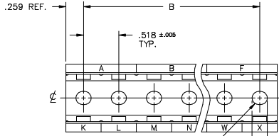
TOP MARKING SCALE - 1:1
