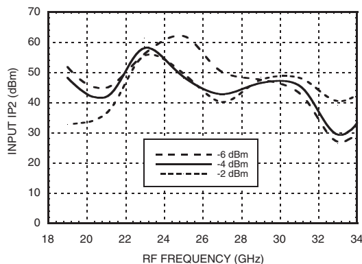
Input IP2 vs. LO Drive @ Vdd = +4V *
