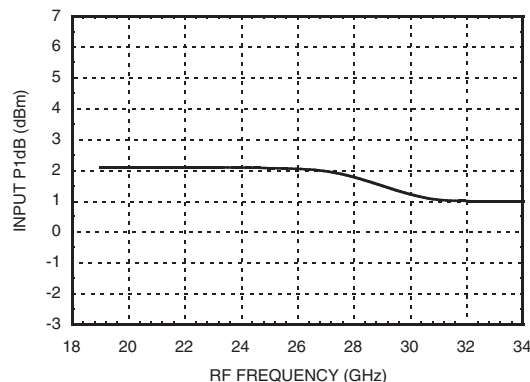
Input P1dB @ LO = -4 dBm, Vdd = +3V
