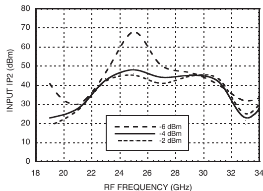
Input IP2 vs. LO Drive @ Vdd = +3V *
