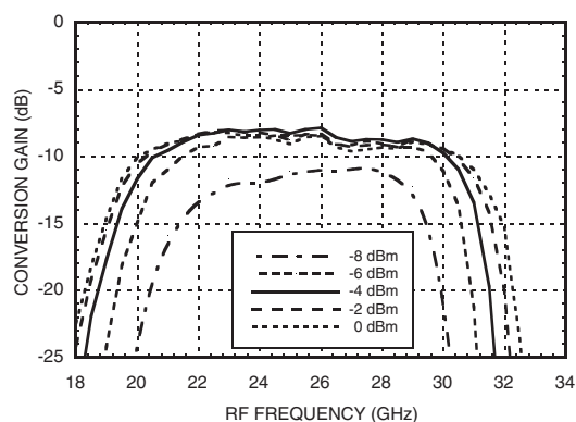
Conversion Gain vs. LO Drive @ Vdd = +3V
