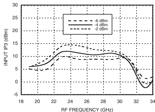
Input IP3 vs. LO Drive @ Vdd = +3V *
