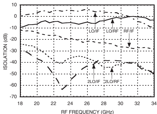
Isolation @ LO = -4 dBm, Vdd = +4V
