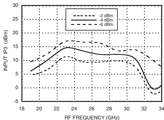
Input IP3 vs. LO Drive @ Vdd = +4V *
