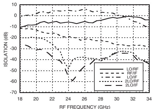
Isolation @ LO = -4 dBm, Vdd = +3V
