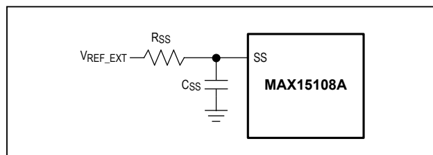
Figure 2. Setting Soft-Start Time
