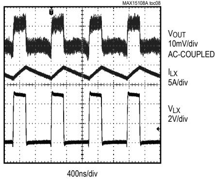
SWITCHING WAVEFORMS ( I_{OUT} = 8\text{A} , V_{IN} = 5\text{V} )
