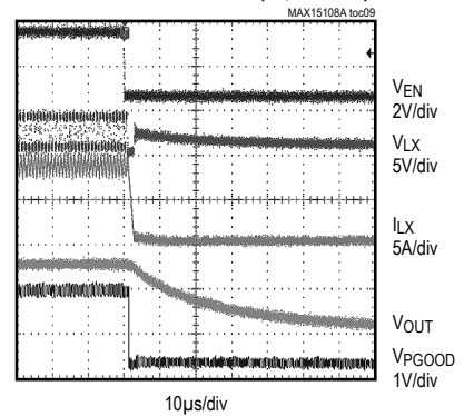
SHUTDOWN WAVEFORM ( I_{LOAD} = 8\text{A} )
