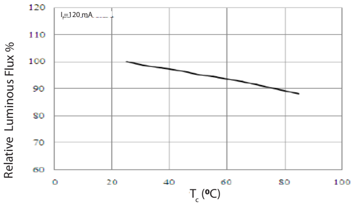
T_c -----Relative Luminous Flux
