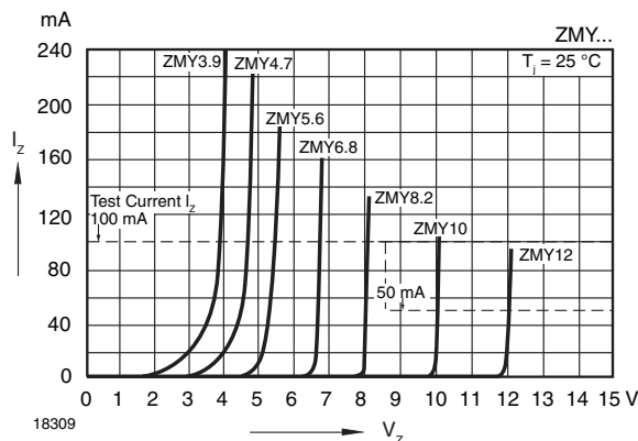
Fig. 6 - Breakdown Characteristics
