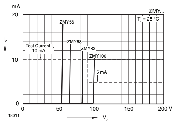
Fig. 8 - Breakdown Characteristics
