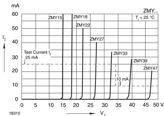
Fig. 7 - Breakdown Characteristics
