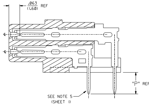
FOR TYPE I 50 CIRCUIT ASSEMBLIES A-71061-2***
