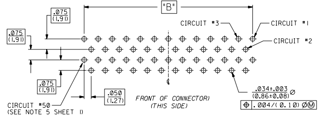
TYPE 150 CIRCUIT P.C.BOARD LAYOUT CONNECTOR SIDE
