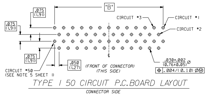
TYPE 1 TAIL P.C.BOARD LAYOUT FOR A-71061-0***
