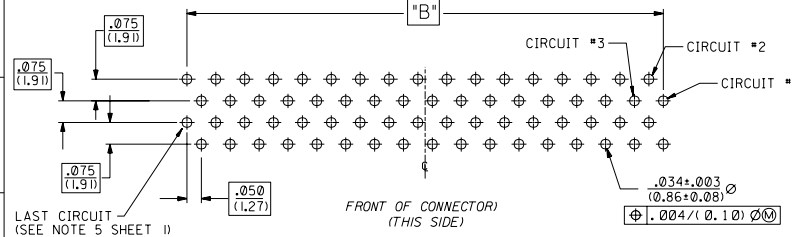
TYPE 1168 CIRCUIT P.C.BOARD LAYOUT CONNECTOR SIDE
