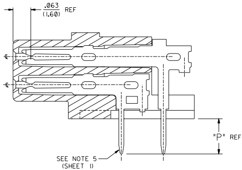
FOR 68 CIRCUIT ASSEMBLIES SECTION A-A A-71061-0***
