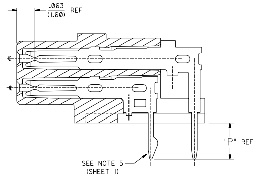
FOR 50 CIRCUIT ASSEMBLIES A-71061-1***
