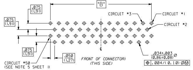
TYPE 150 CIRCUIT P.C. BOARD LAYOUT CONNECTOR SIDE
