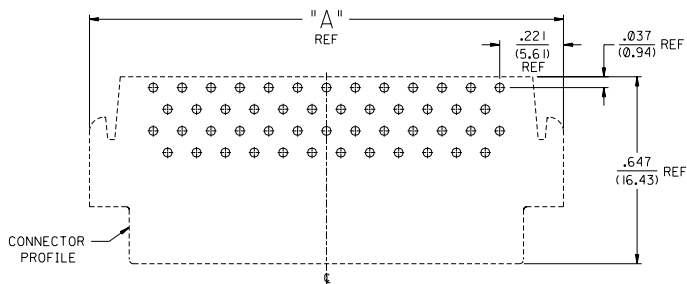
RECOMMENDED CONNECTOR LAYOUT (50 CKT SHOWN FOR REFERENCE)
