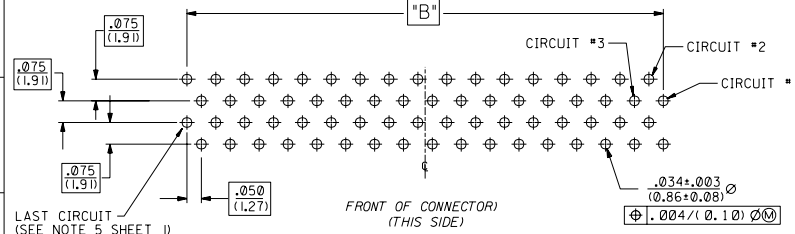
TYPE 1168 CIRCUIT P.C. BOARD LAYOUT CONNECTOR SIDE
