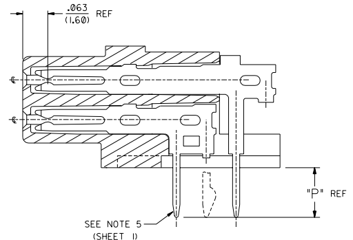
FOR 68 CIRCUIT ASSEMBLIES SECTION A-A FOR RETENTION TAIL OPTION A-71061-1***
