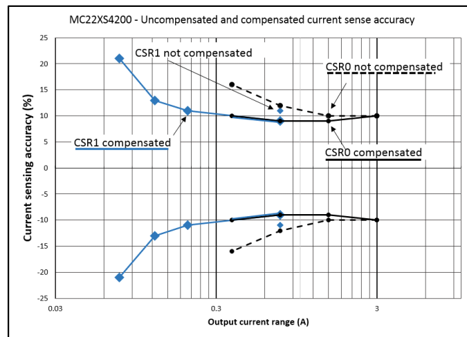
Figure 19. Current Sense Accuracy Versus Output Current
