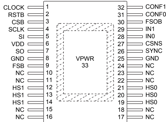
Figure 3. Device Pin Assignments
