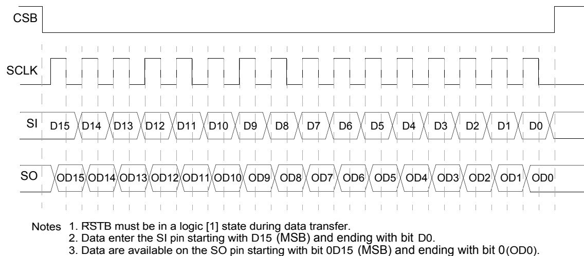
Figure 21. 16-Bit SPI Interface Timing Diagram
