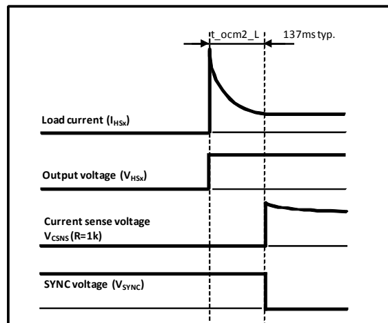
Figure 13. Current Sense Blanking During Overcurrent Window Activity
