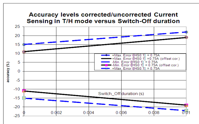
Figure 20. Track and Hold Current Sense Accuracy
