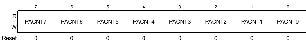
Figure 8-27. Pulse Accumulator Count Register Low (PACNT7-0)
