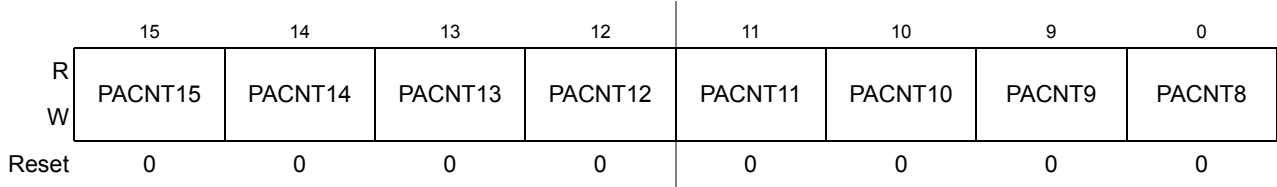
Figure 8-26. Pulse Accumulator Count Register High (PACNT15-8)
