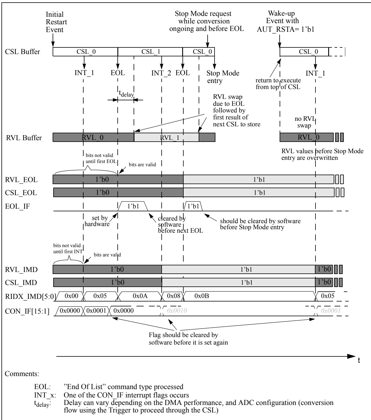
Figure 10-40. RVL Swapping — Use Case Diagram
