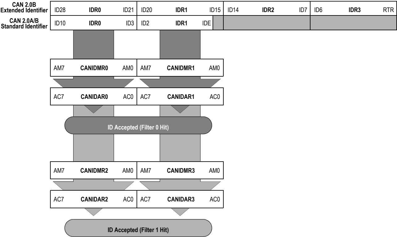
Figure 11-41. 16-bit Maskable Identifier Acceptance Filters
