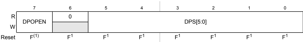
Figure 21-15. EEPROM Protection Register (DFPROT)
