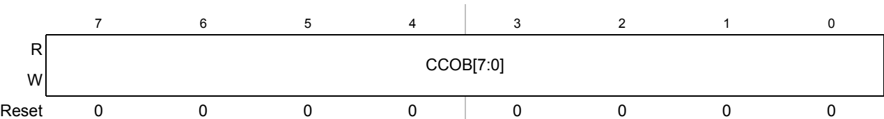
Figure 21-21. Flash Common Command Object 1 Low Register (FCCOB1LO)
