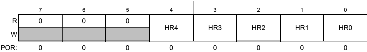
Figure 18-12. Hour Register (HRR)
