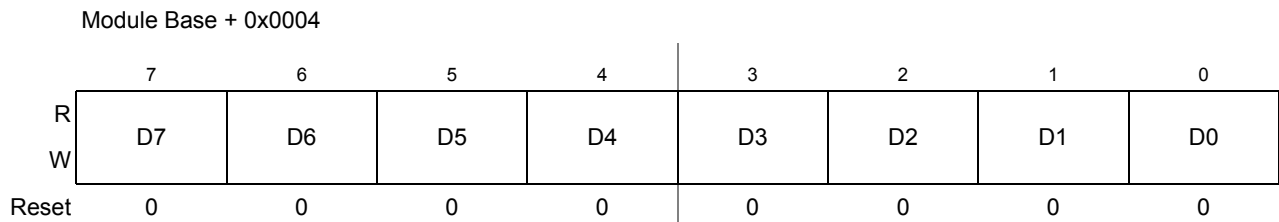
Figure 14-8. IIC Bus Data I/O Register (IBDR)
