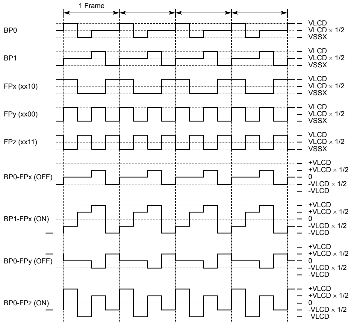
Figure 15-12. 1/2 Duty and 1/2 Bias
