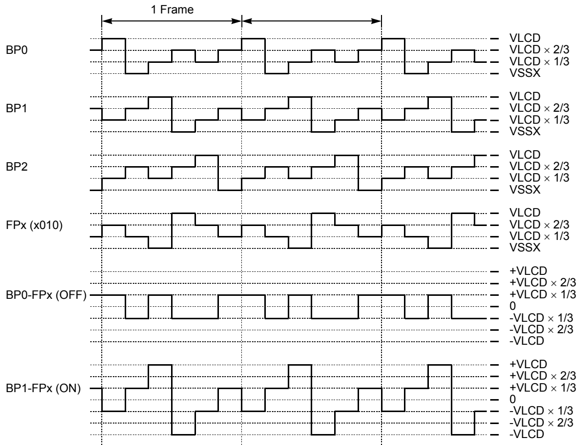
Figure 15-14. 1/3 Duty and 1/3 Bias
