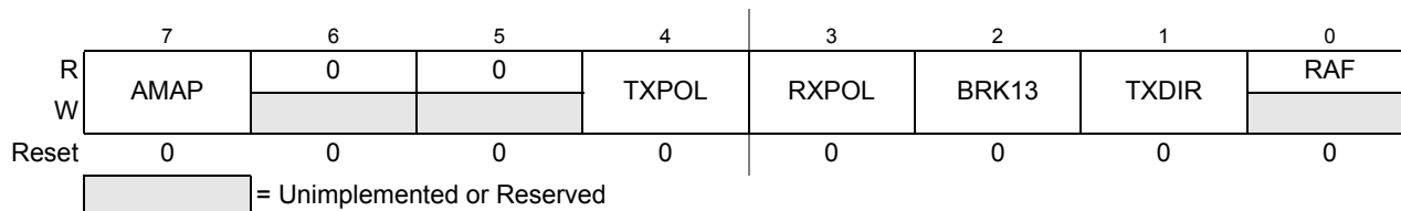
Figure 12-11. SCI Status Register 2 (SCISR2)
