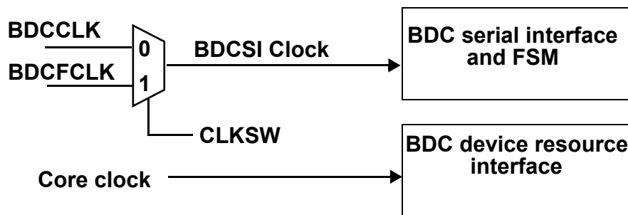
Figure 5-5. Clock Switch
