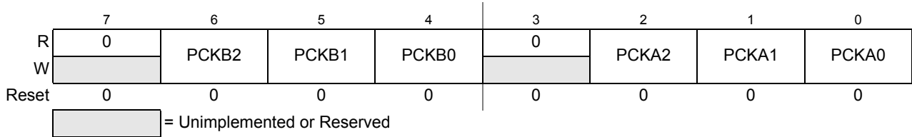
Figure 9-6. PWM Prescale Clock Select Register (PWMPRCLK)
