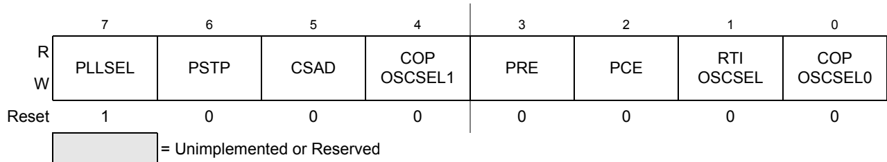
Figure 7-10. S12CPMU_UHV_V5 Clock Select Register (CPMUCLKS)
