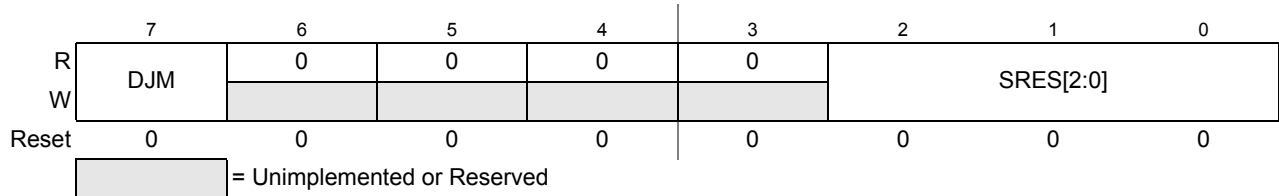
Figure 10-8. ADC Format Register (ADCFMT)
