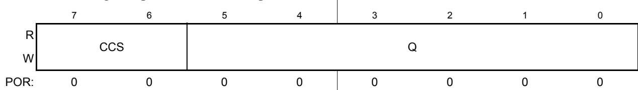
Figure 18-7. RTC Compensation Configure Register (RTCCCR)
