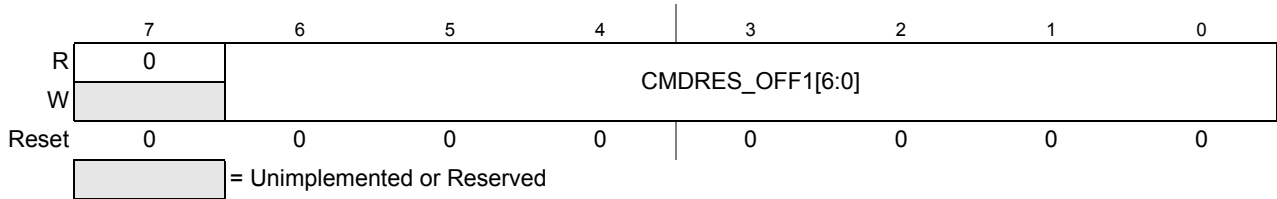
Figure 10-27. ADC Command and Result Offset Register 1 (ADCCROFF1)
