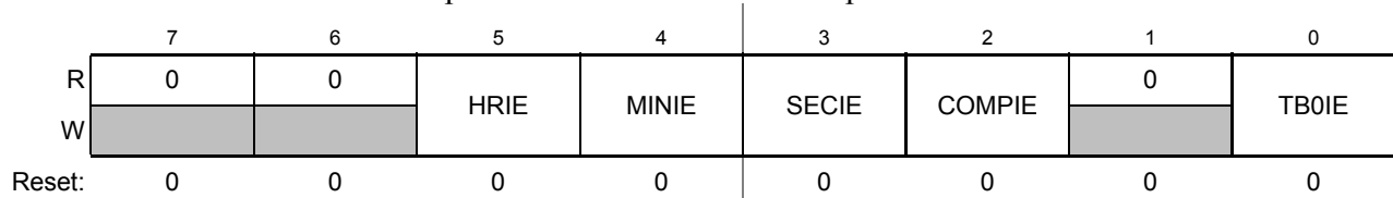
Figure 18-5. RTC Control Register 4 (RTCCTL4)
