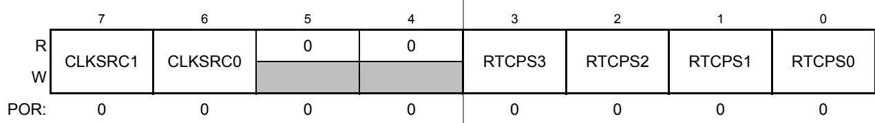
Figure 18-3. RTC Control Register 2(RTCCTL2)
