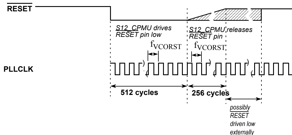
Figure 7-40. RESET Timing
