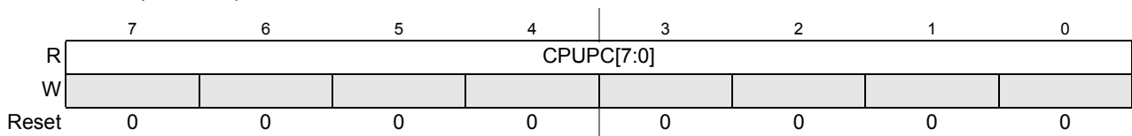
Figure 3-7. Captured S12ZCPU Program Counter (MMCPCH, MMCPCH, MMCPCH)
