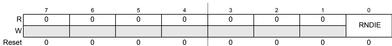
Figure 19-16. SSG Interrupt Enable Register (SSGIE)
