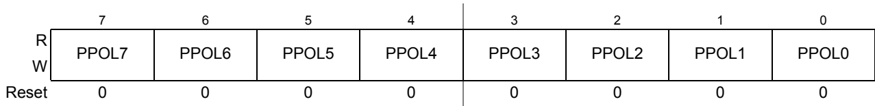
Figure 9-4. PWM Polarity Register (PWMPOL)
