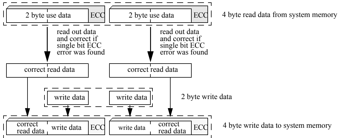
Figure 20-9. 2 byte non-aligned write access
