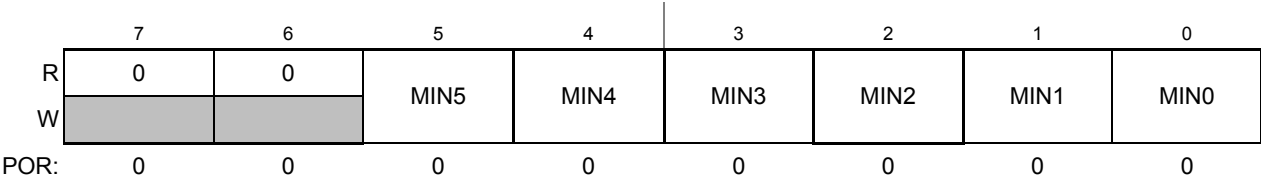
Figure 18-11. Minute Register (MINR)
