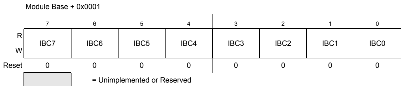
Figure 14-4. IIC Bus Frequency Divider Register (IBFD)
