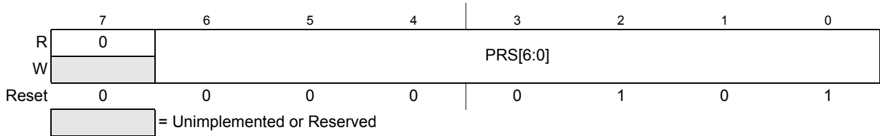
Figure 10-7. ADC Timing Register (ADCTIM)
