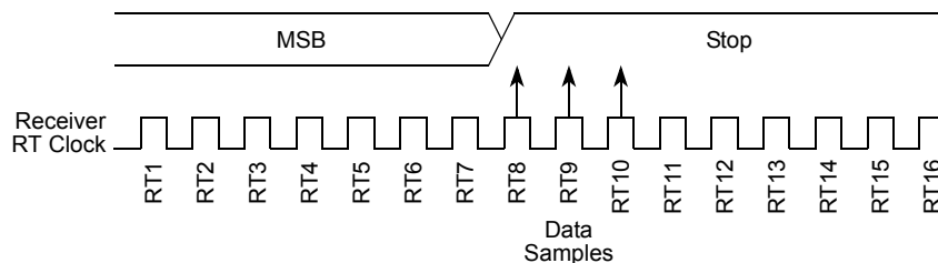
Figure 12-28. Slow Data
