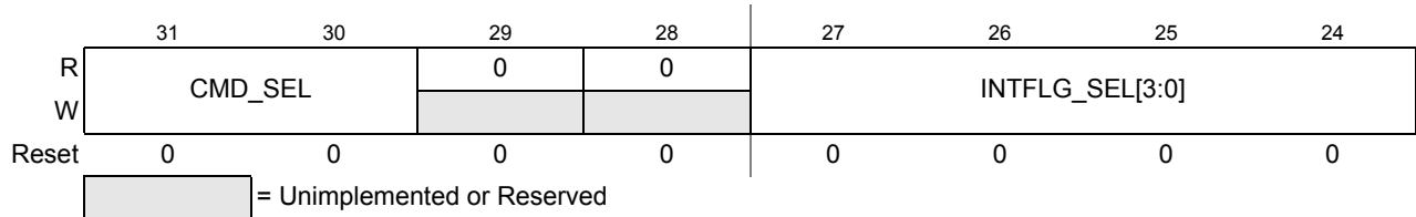
Figure 10-18. ADC Command Register 0 (ADCCMD_0)
