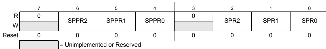
Figure 13-5. SPI Baud Rate Register (SPIBR)
