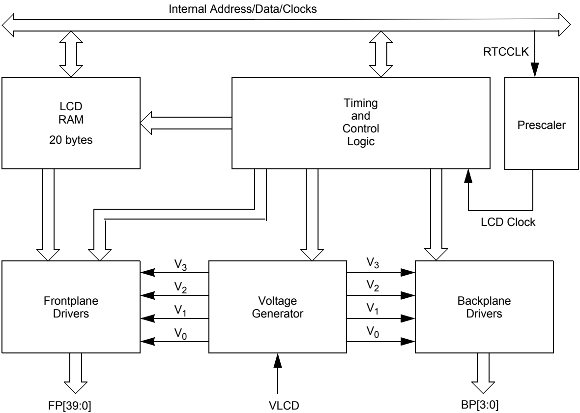
Figure 15-1. LCD40F4BV3 Block Diagram
