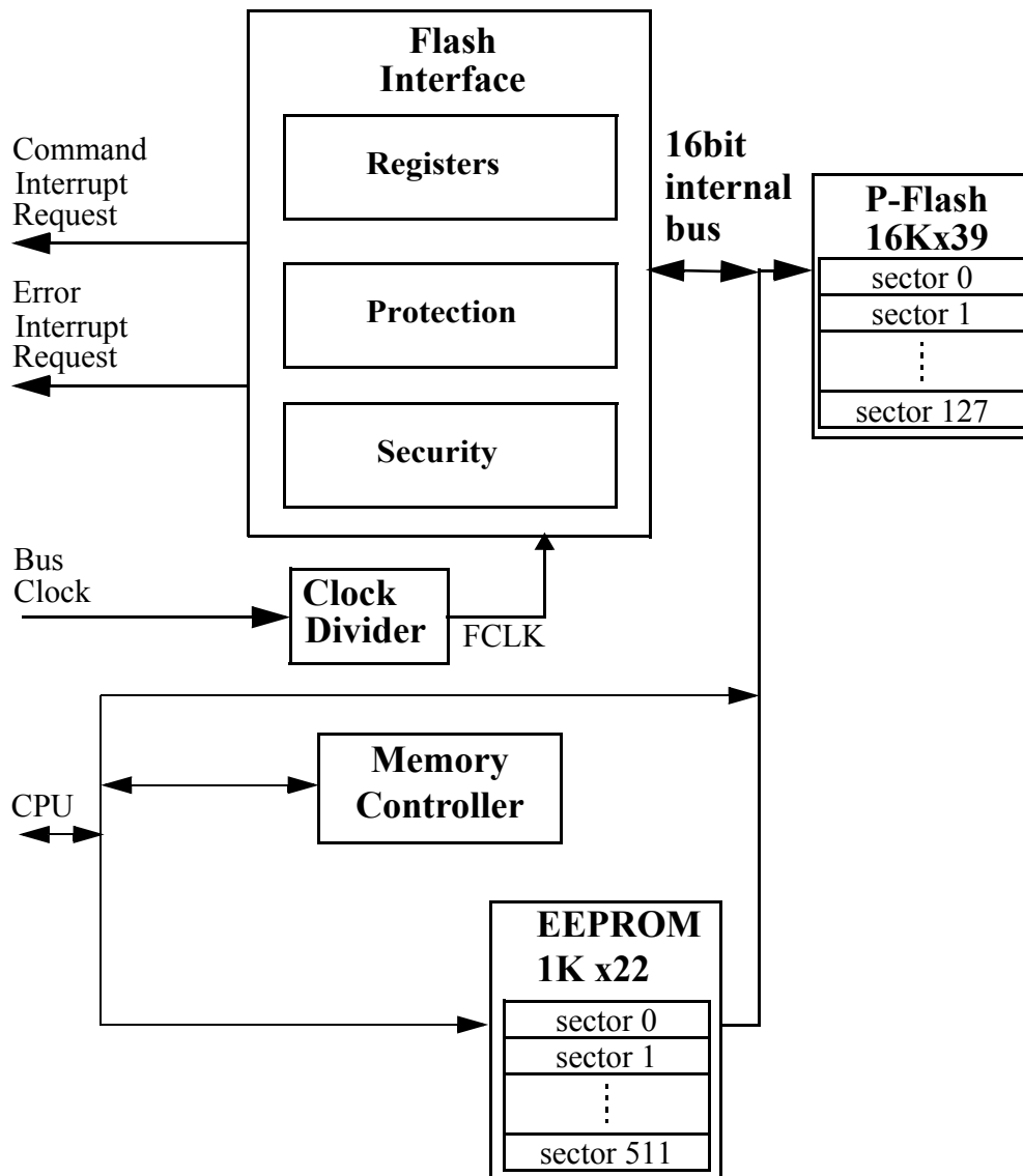
Figure 21-1. FTMRZ64K2K Block Diagram
