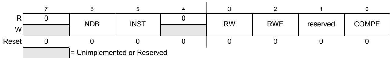
Figure 6-14. Debug Comparator A Control Register
