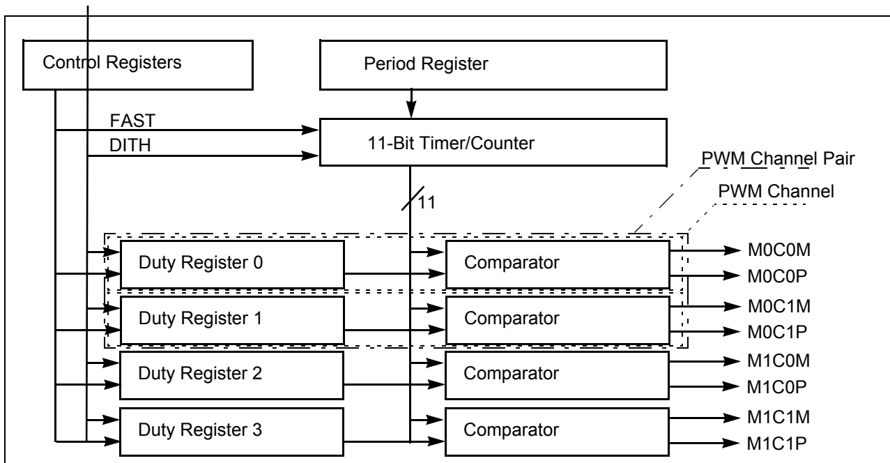
Figure 16-1. MC10B8C Block Diagram
