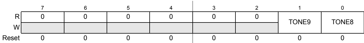
Figure 19-7. SSG Tone Register (SSGTONEH)
