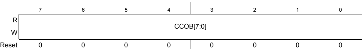
Figure 21-19. Flash Common Command Object 0 Low Register (FCCOB0LO)
