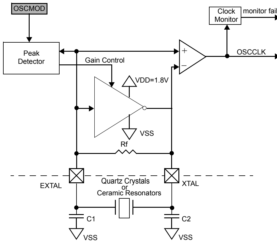
Figure 7-2. XOSCLCP Block Diagram
