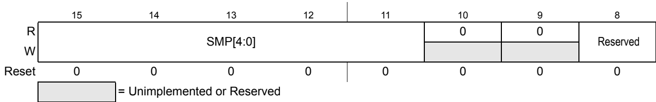
Figure 10-20. ADC Command Register 2 (ADCCMD_2)
