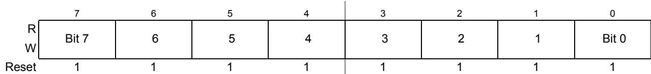
Figure 9-13. PWM Channel Period Registers (PWMPERx)
