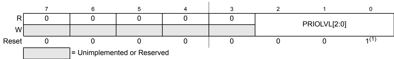
Figure 4-12. Interrupt Request Configuration Data Register 7 (INT_CFDATA7)
