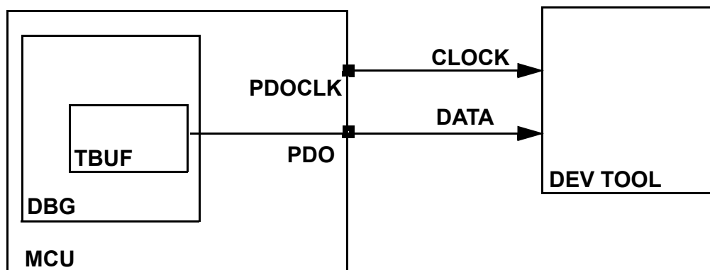
Figure 6-30. Profiling Output Interface
