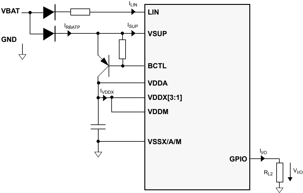
Figure A-2. Supply Currents Overview
