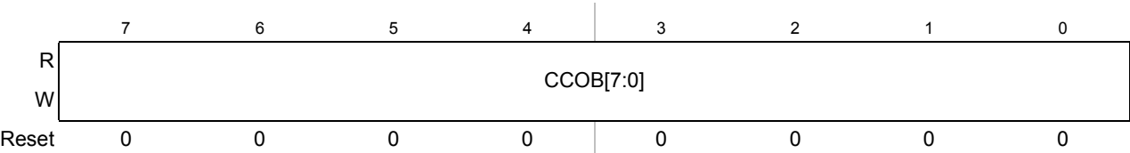
Figure 21-29. Flash Common Command Object 5 Low Register (FCCOB5LO)
