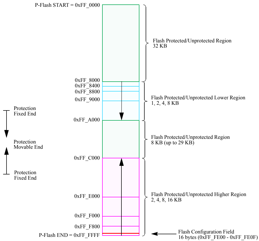
Figure 21-2. P-Flash Memory Map
