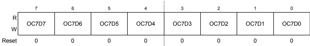
Figure 8-9. Output Compare 7 Data Register (OC7D)
