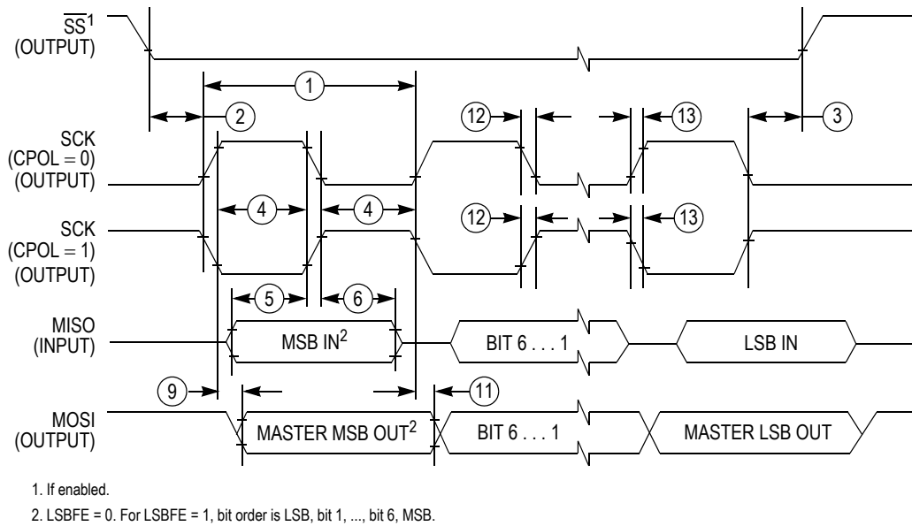
Figure L-2. SPI Master Timing (CPHA=1)
