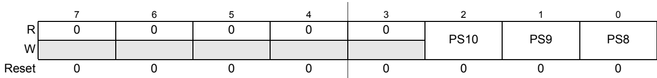
Figure 19-5. SSG Clock Prescaler Register (SSGPSH)
