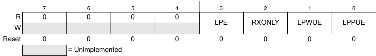
Figure 23-4. LIN Control Register (LPCR)
