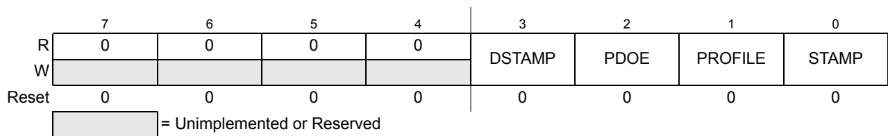
Figure 6-6. Debug Trace Control Register Low (DBGTCRL)
