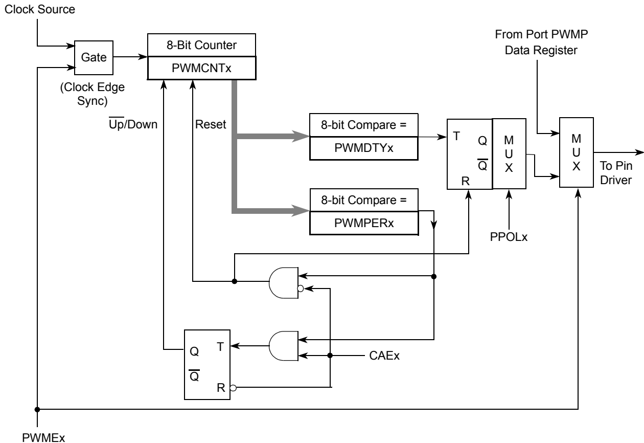
Figure 9-16. PWM Timer Channel Block Diagram
