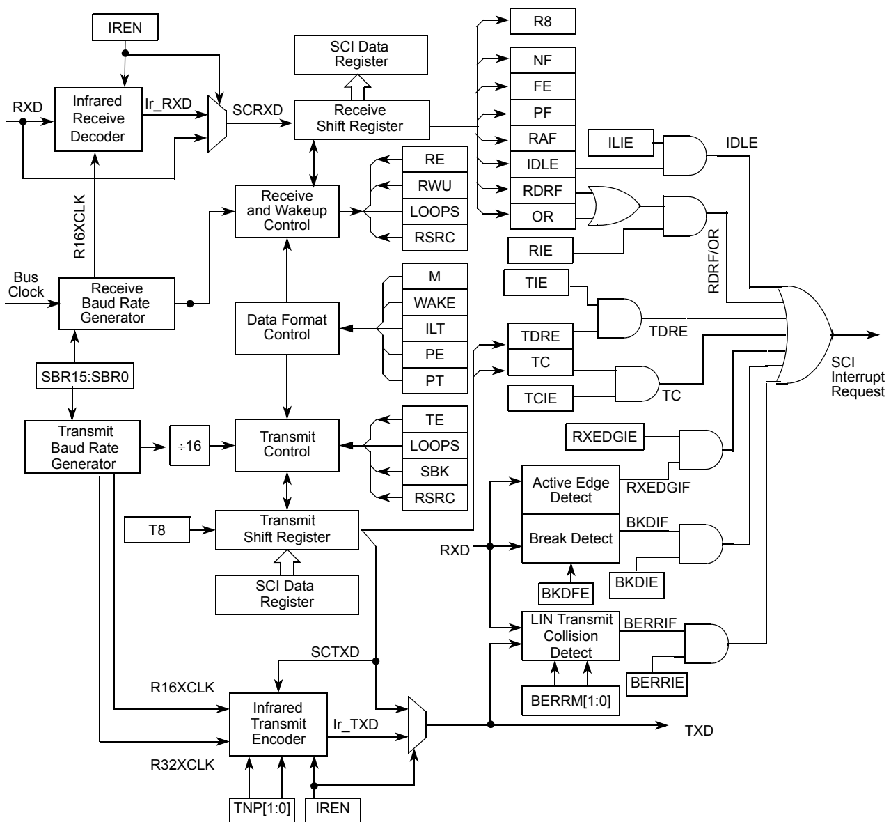
Figure 12-14. Detailed SCI Block Diagram
