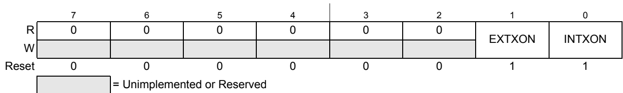
Figure 7-34. Voltage Regulator Control Register (CPMUVREGCTL)
