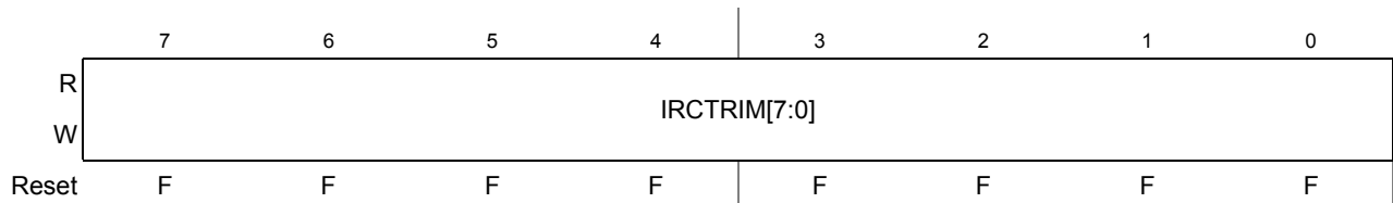
Figure 7-28. S12CPMU_UHV_V5 IRC1M Trim Low Register (CPMUIRCTRIML)
