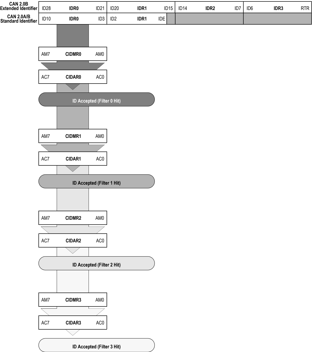
Figure 11-42. 8-bit Maskable Identifier Acceptance Filters
