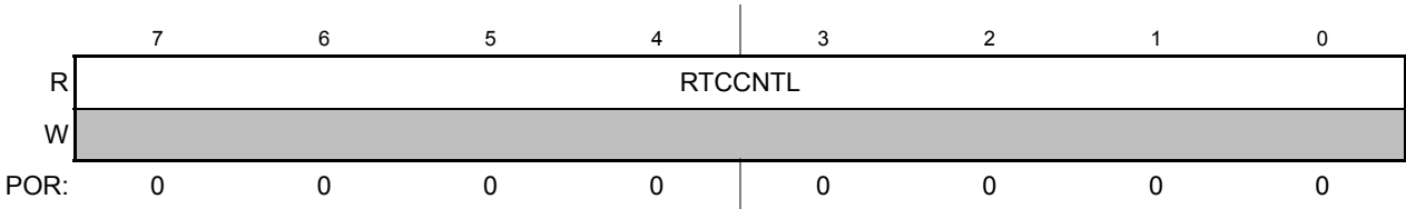
Figure 18-8. RTC Counter Register (RTCCNT)
