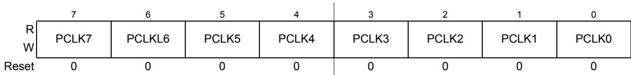
Figure 9-5. PWM Clock Select Register (PWMCLK)
