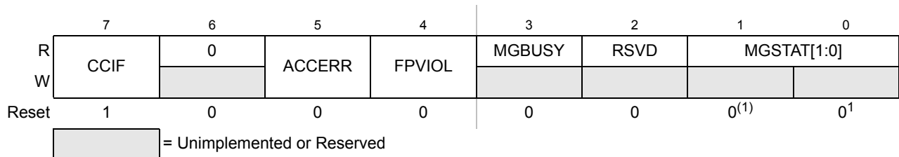
Figure 21-11. Flash Status Register (FSTAT)
