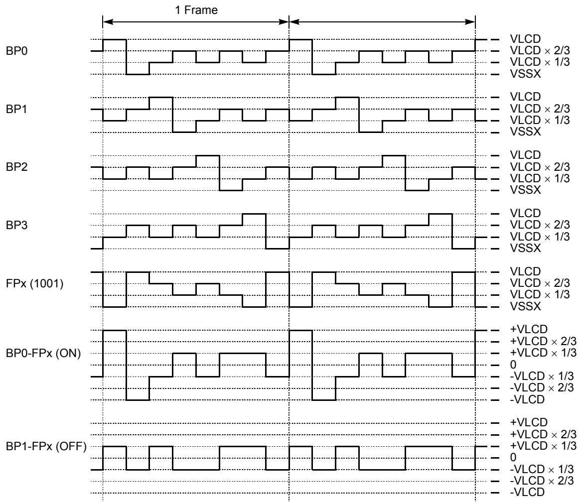
Figure 15-15. 1/4 Duty and 1/3 Bias
