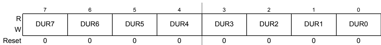
Figure 19-15. SSG Tone Duration Register (SSGDUR)
