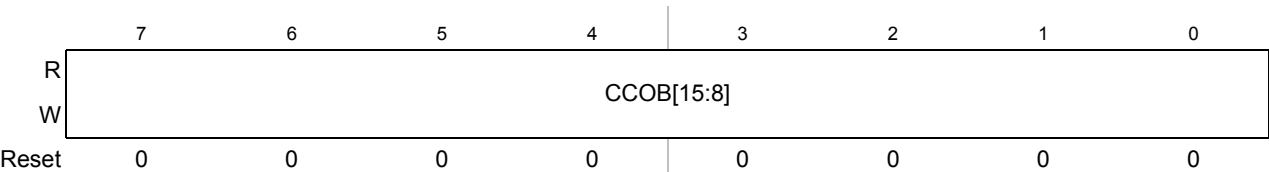
Figure 21-22. Flash Common Command Object 2 High Register (FCCOB2HI)
