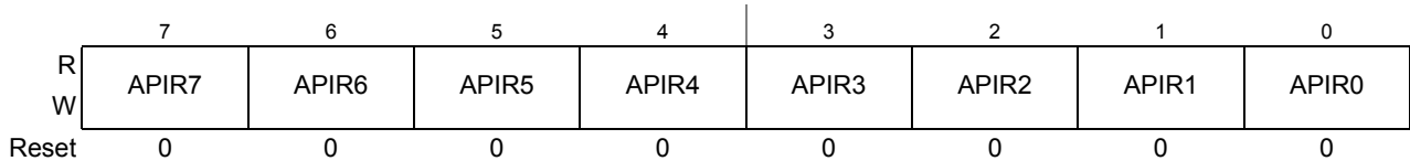
Figure 7-24. Autonomous Periodical Interrupt Rate Low Register (CPMUAPIRL)
