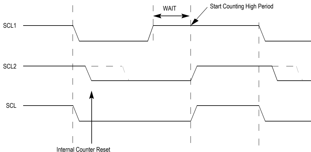
Figure 14-12. IIC-Bus Clock Synchronization
