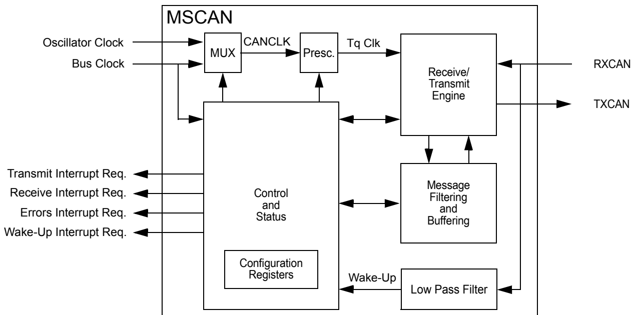
Figure 11-1. MSCAN Block Diagram
