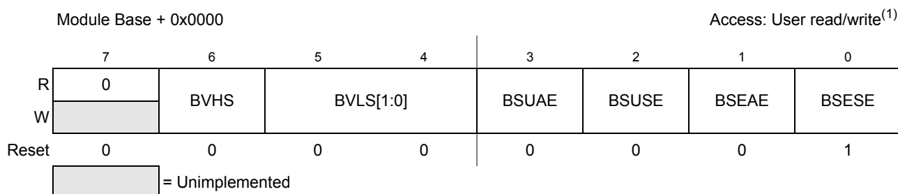
Figure 22-3. BATS Module Enable Register (BATE)
