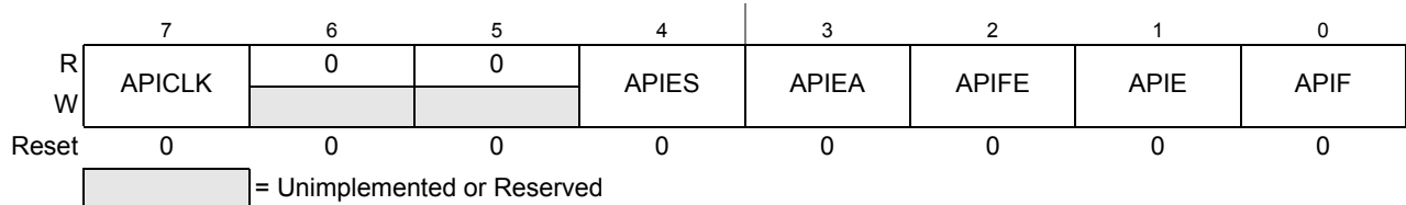
Figure 7-20. Autonomous Periodical Interrupt Control Register (CPMUAPICTL)
