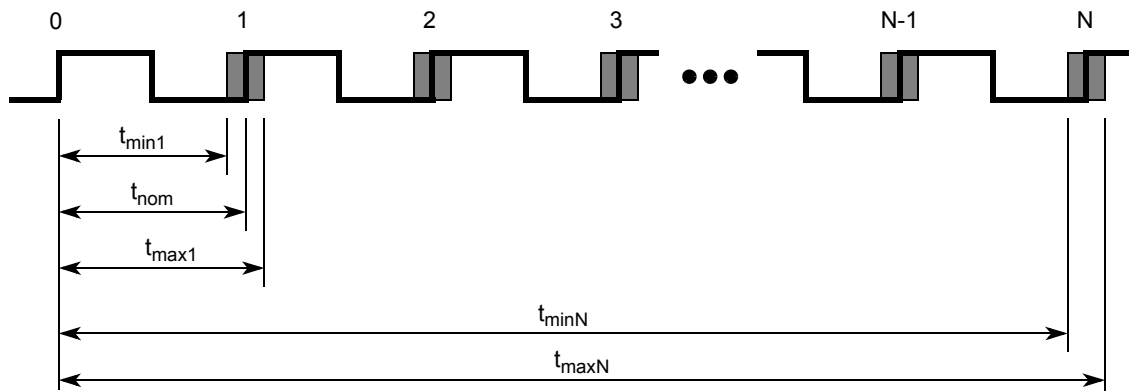
Figure C-1. Jitter Definitions
