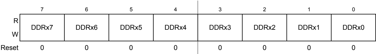
Figure 2-15. Data Direction Register
