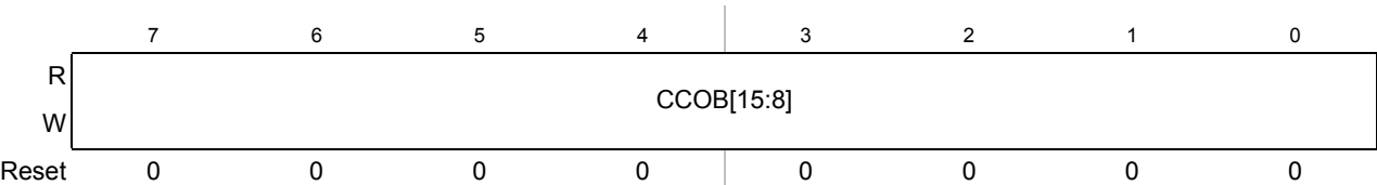
Figure 21-20. Flash Common Command Object 1 High Register (FCCOB1HI)
