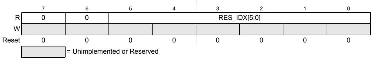
Figure 10-24. ADC Result Index Register (ADCRIDX)
