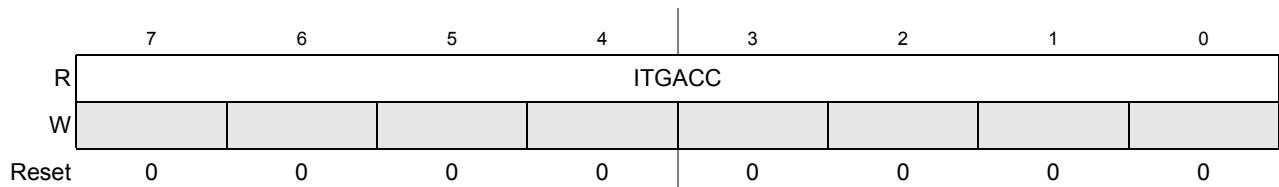
Figure 17-9. Integration Accumulator Register Low (ITGACC)
