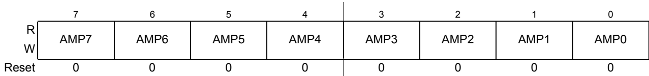
Figure 19-10. SSG amplitude Register (SSGAMPL)
