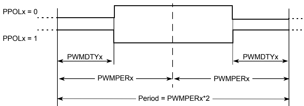
Figure 9-19. PWM Center Aligned Output Waveform
