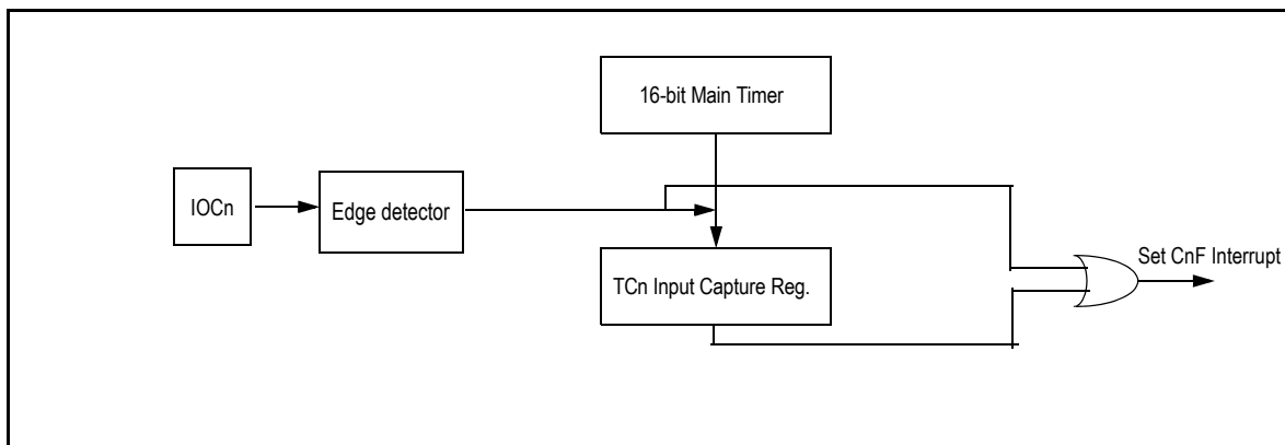
Figure 8-3. Interrupt Flag Setting
