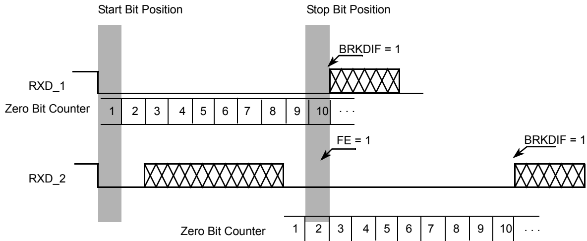
Figure 12-17. Break Detection if BRKDFE = 1 (M = 0)
