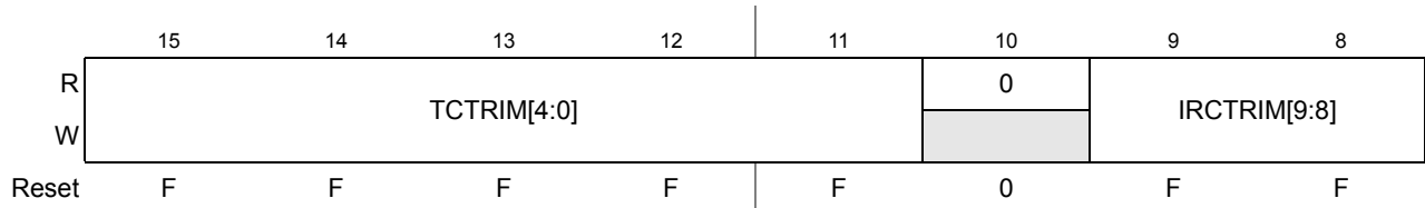
Figure 7-27. S12CPMU_UHV_V5 IRC1M Trim High Register (CPMUIRCTRIMH)
