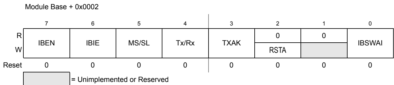
Figure 14-6. IIC Bus Control Register (IBCR)
