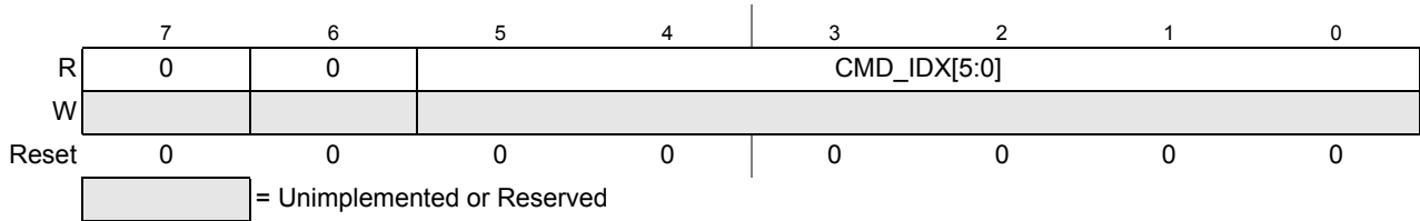
Figure 10-22. ADC Command Index Register (ADCCIDX)
