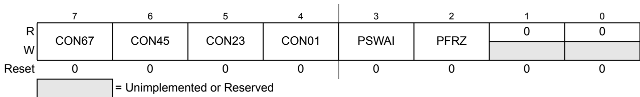
Figure 9-8. PWM Control Register (PWMCTL)
