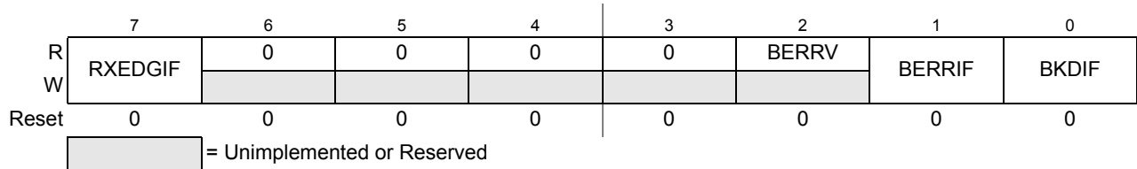
Figure 12-6. SCI Alternative Status Register 1 (SCIASR1)
