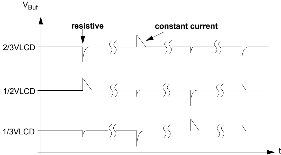
Figure E-2. V_{Buf} transients (not to scale)
