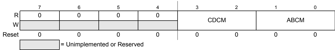
Figure 6-4. Debug Control Register2 (DBGCR2)
