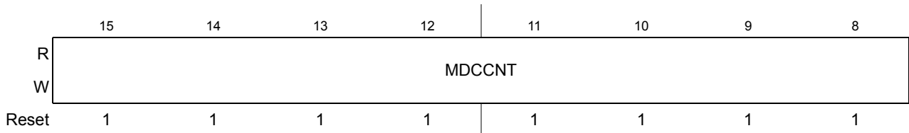
Figure 17-6. Modulus Down-Counter Count Register High (MDCCNT)
