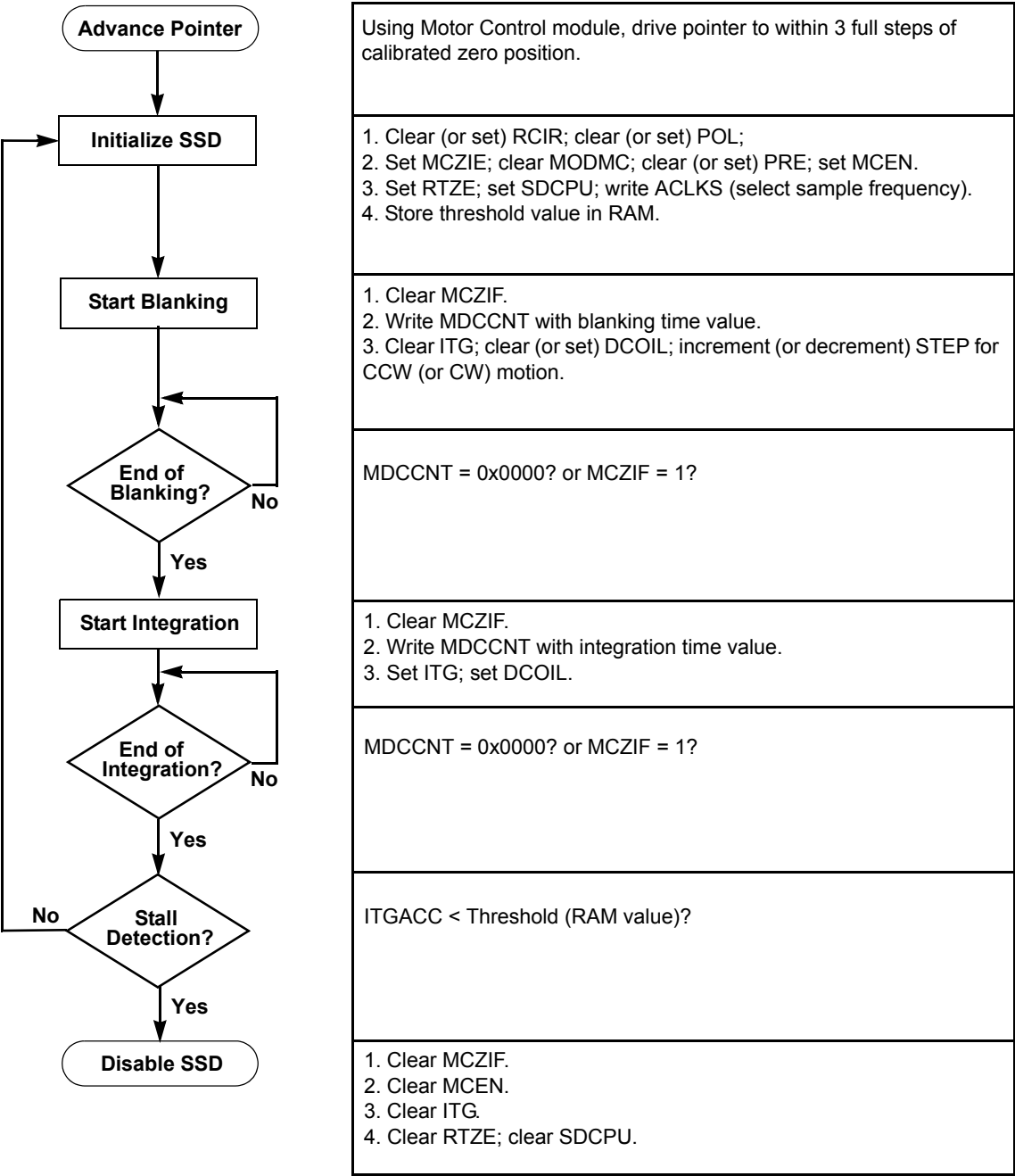
Figure 17-15. Return-to-Zero Flowchart
