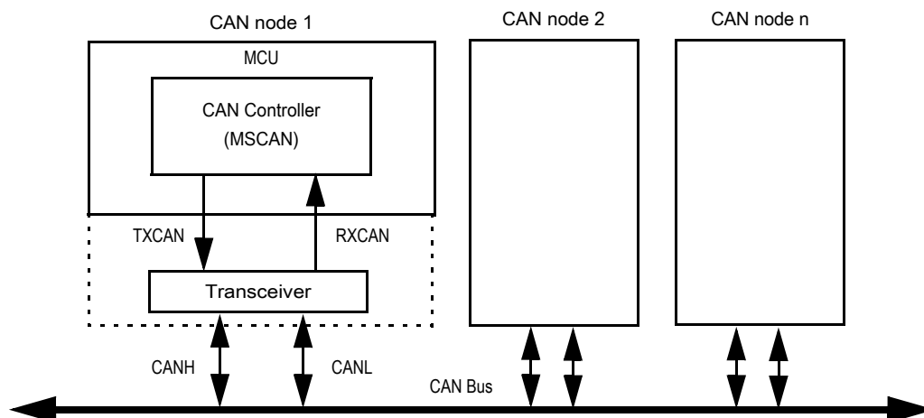
Figure 11-2. CAN System
