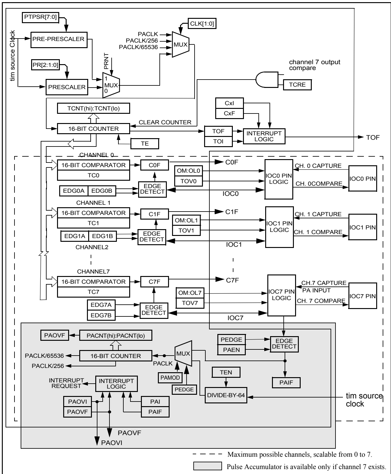
Figure 8-30. Detailed Timer Block Diagram
