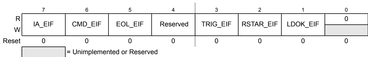
Figure 10-12. ADC Error Interrupt Flag Register (ADCEIF)
