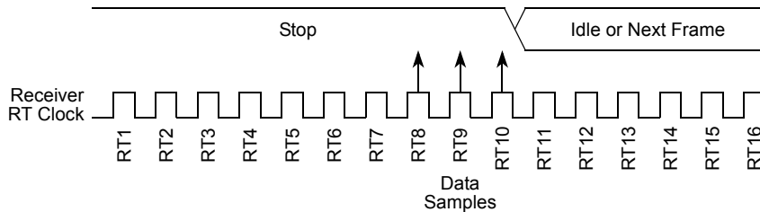
Figure 12-29. Fast Data
