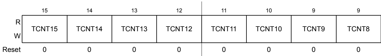
Figure 8-10. Timer Count Register High (TCNTH)
