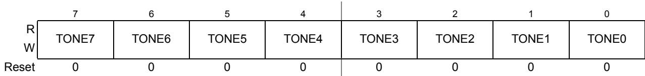
Figure 19-8. SSG Tone Register (SSGTONEL)
