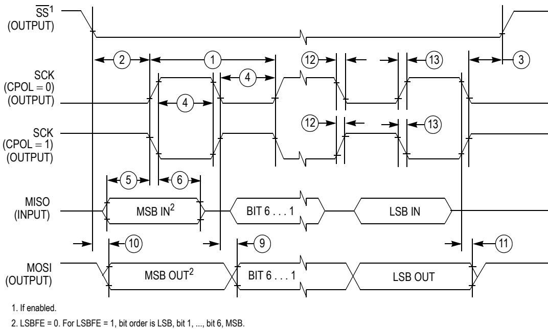
Figure L-1. SPI Master Timing (CPHA=0)
