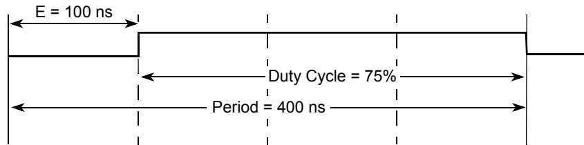
Figure 9-18. PWM Left Aligned Output Example Waveform
