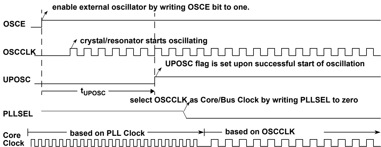
Figure 7-39. Enabling the external oscillator
