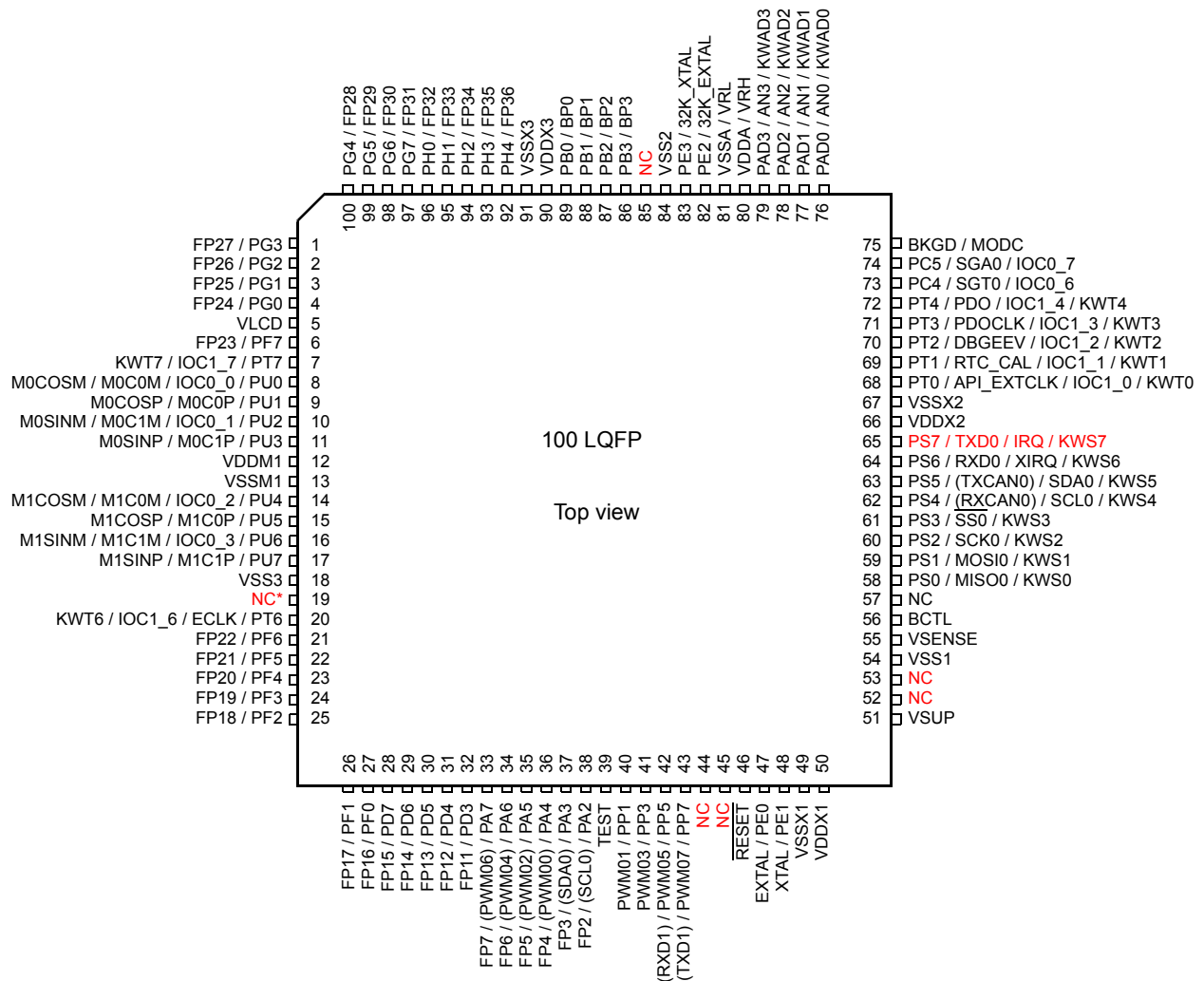
Figure 1-5. MC9S12ZVHY 100-pin LQFP pin out
