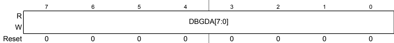
Figure 6-25. Debug Comparator D Address Register
