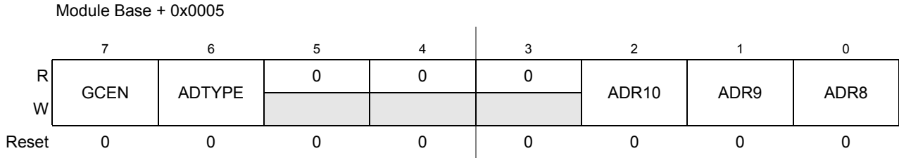
Figure 14-9. IIC Bus Control Register 2(BCR2)
