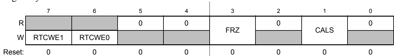
Figure 18-4. RTC Control Register 3(RTCCTL3)
