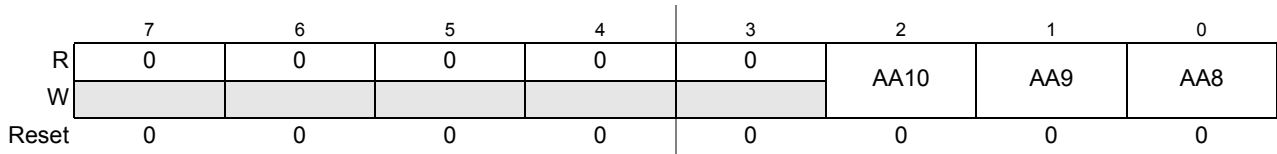
Figure 19-11. SSG Amplitude Adjustment (SSGAH)
