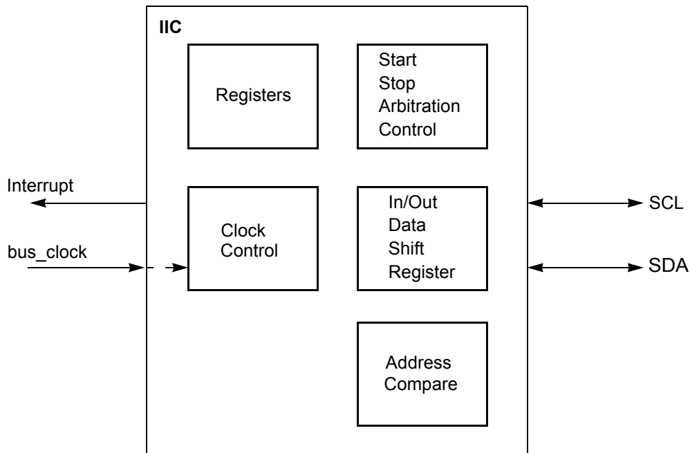
Figure 14-1. IIC Block Diagram
