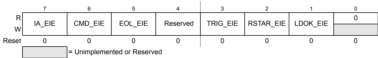
Figure 10-10. ADC Error Interrupt Enable Register (ADCEIE)
