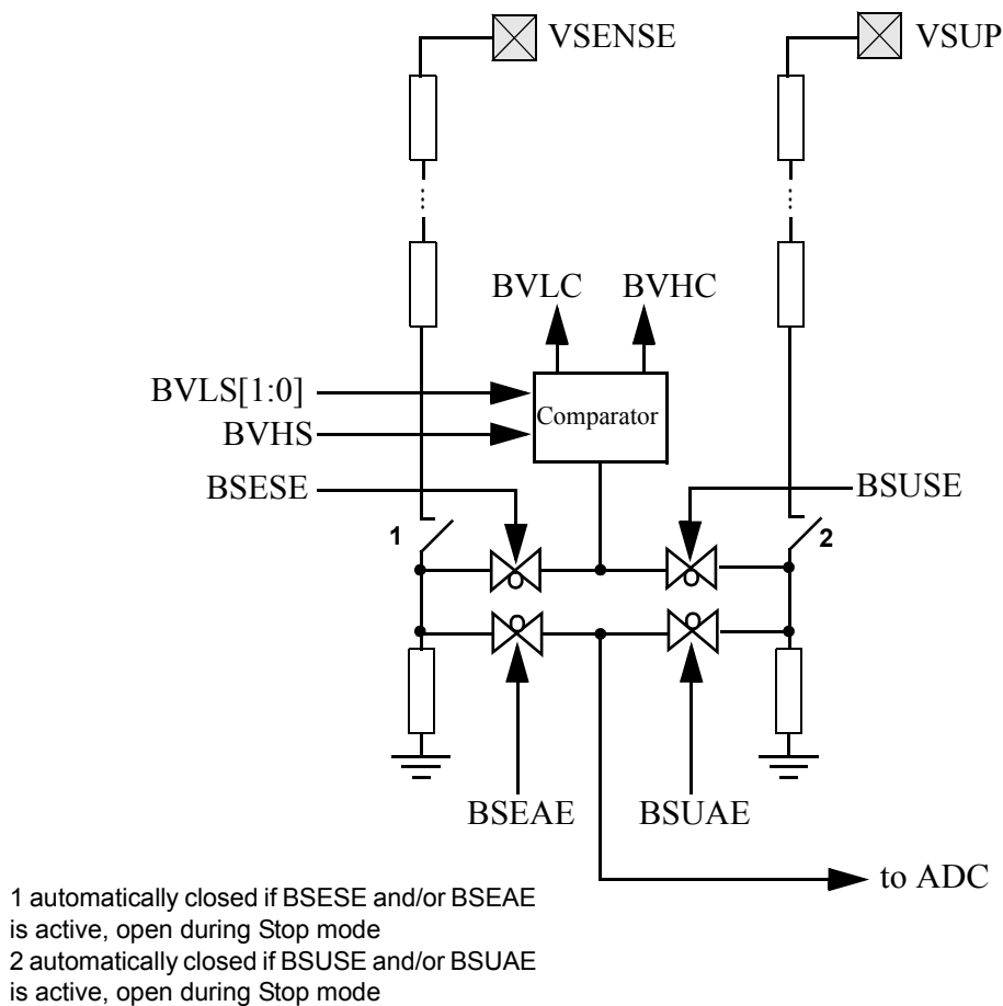
Figure 22-1. BATS Block Diagram
