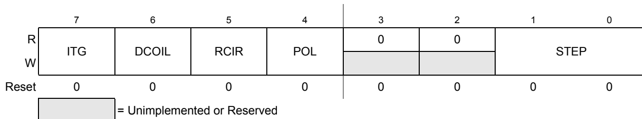
Figure 17-2. Return-to-Zero Control Register (RTZCTL)
