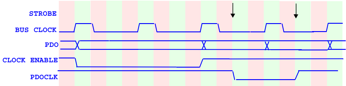
Figure 6-31. PDO Profiling Clock Control
