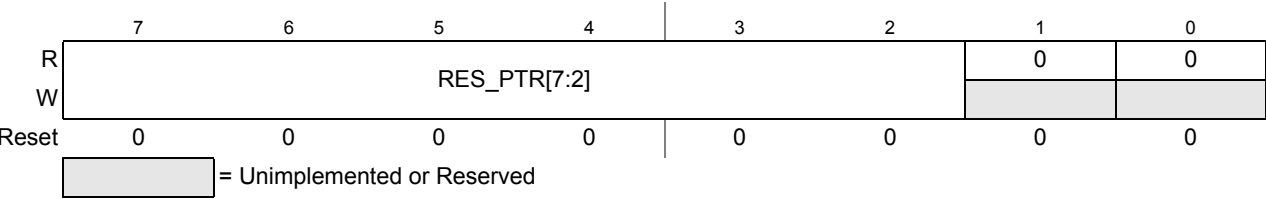
Figure 10-25. ADC Result Base Pointer Registers (ADCRBP_0, ADCRBP_1, ADCRBP_2)
