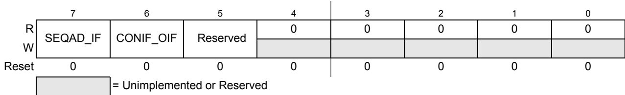
Figure 10-13. ADC Interrupt Flag Register (ADCIF)
