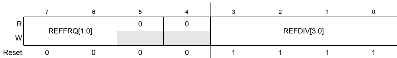
Figure 7-6. S12CPMU_UHV_V5 Reference Divider Register (CPMUREFDIV)
