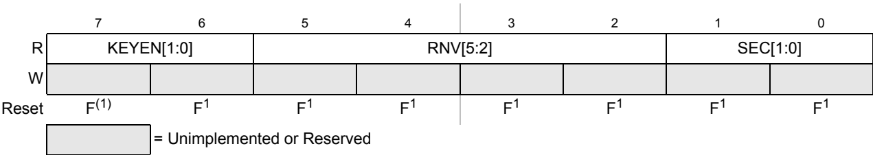
Figure 21-6. Flash Security Register (FSEC)
