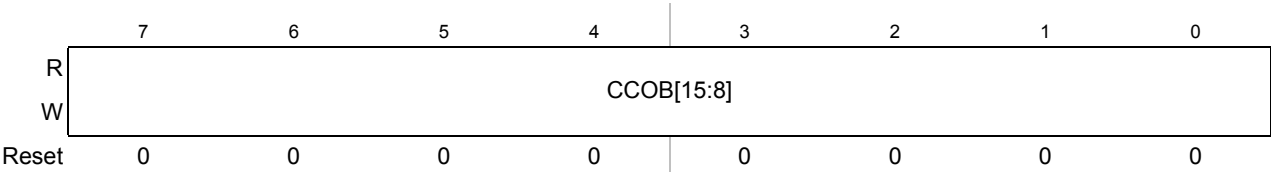
Figure 21-24. Flash Common Command Object 3 High Register (FCCOB3HI)
