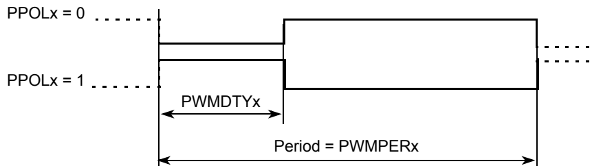
Figure 9-17. PWM Left Aligned Output Waveform
