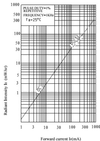
Fig.2 Radiant Intensity vs. Forward Current
