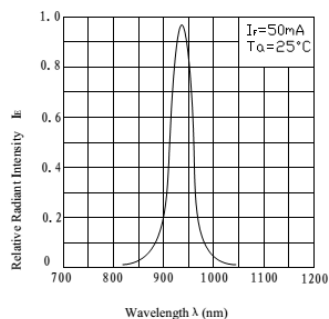
Fig.5 Relative Radiant Intensity vs. Wavelength
