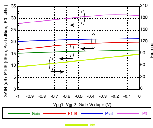
Gain, Power & Output IP3 vs. Gate Voltage @ 12 GHz
