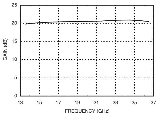
Linear Gain vs. Frequency
