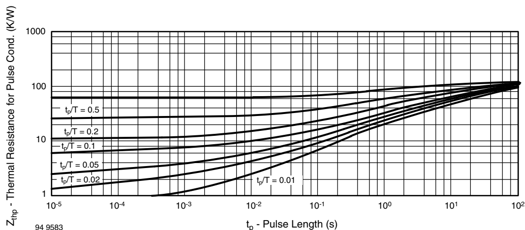
Fig. 5 - Thermal Response
