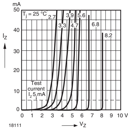
Fig. 14 - Breakdown Characteristics
