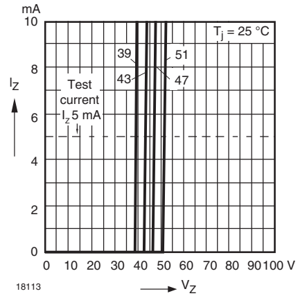
Fig. 16 - Breakdown Characteristics
