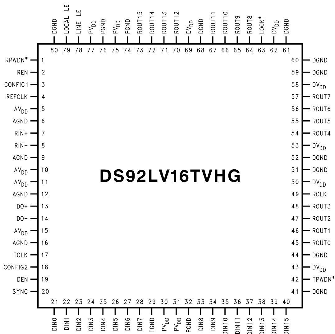
Figure 22. DS92LV16TVHG (Top View)
