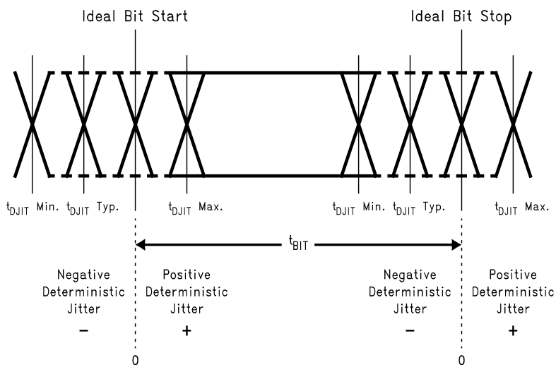
Figure 16. Deterministic Jitter and Ideal Bit Position
