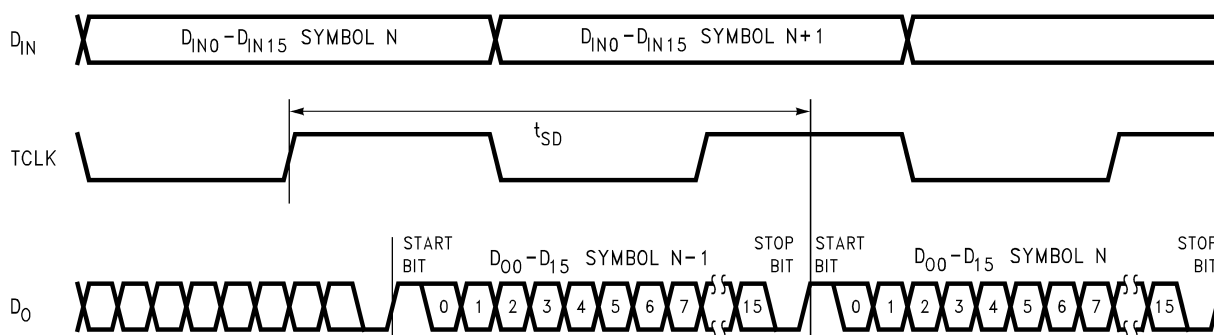
Figure 10. Serializer Delay
