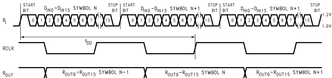
Figure 11. Deserializer Delay
