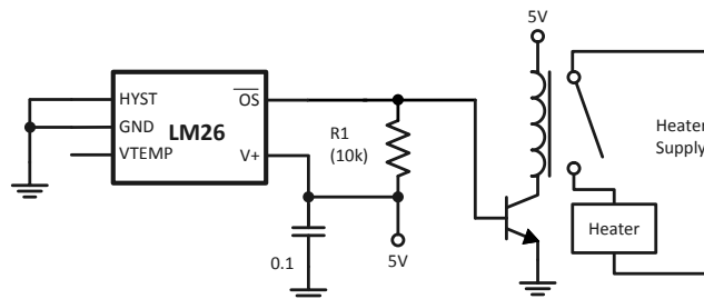
Figure 13. Simple Thermostat
