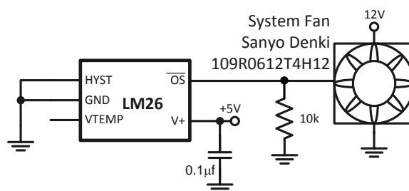
Figure 8. Two-Speed Fan Speed Control
