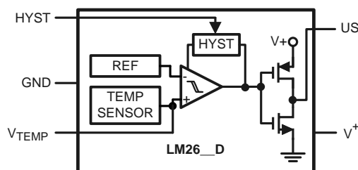
Figure 5. LM26-__D Output Pin Block Diagram
