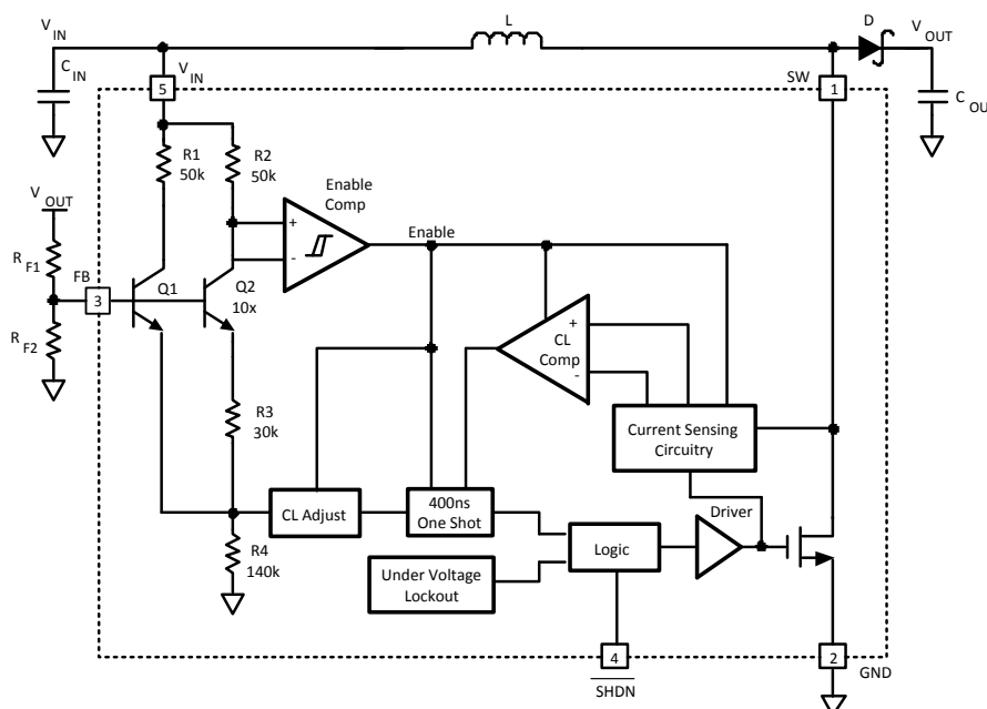
Figure 15. LM2703 Block Diagram
