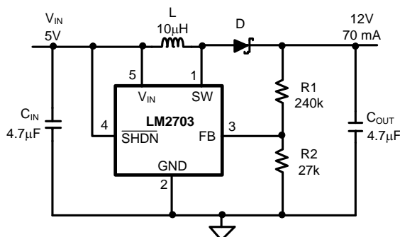
Figure 20. 5V to 12V Application
