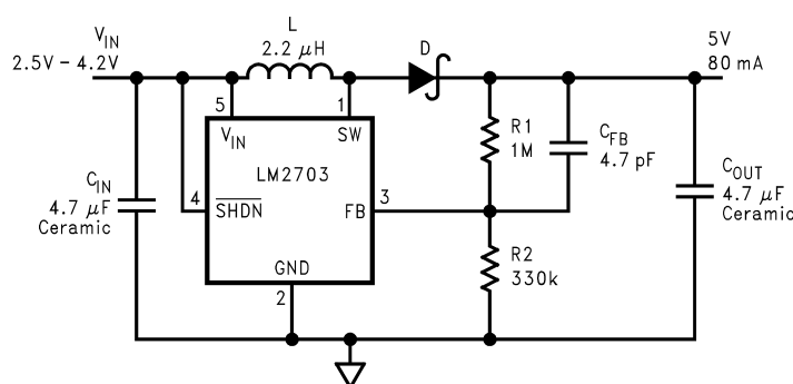
Figure 18. Li-Ion 5V Application
