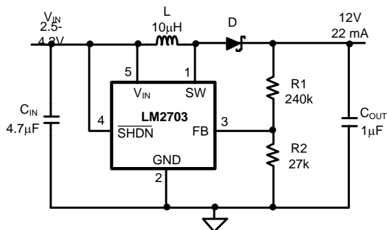
Figure 19. Li-Ion 12V Application
