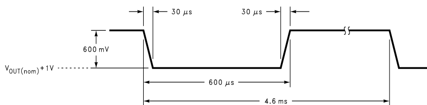
Figure 1. Line Regulation Input Test Signal
