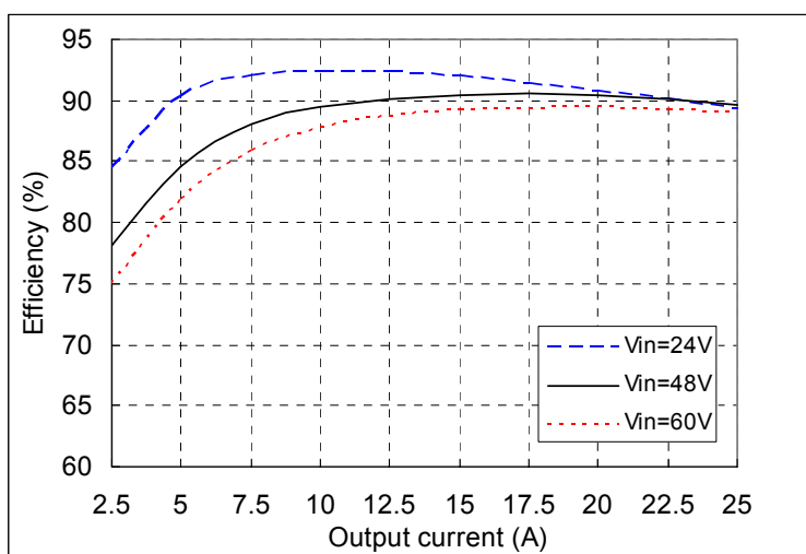
Figure 1 Efficiency vs. output current, T_a=25^{\circ}\text{C} , V_o=3.3\text{V}
