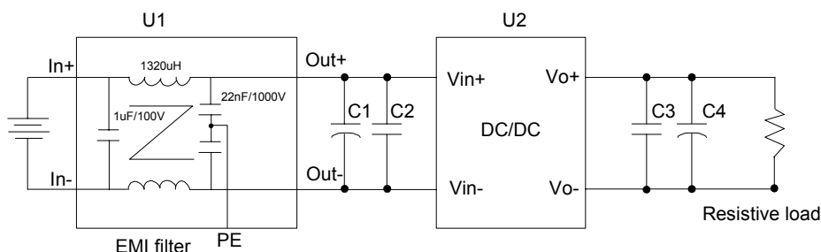
Figure 15 EMC test configuration
