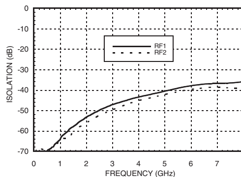
Isolation
