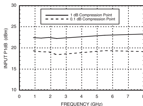
0.1 and 1 dB Input Compression Point
