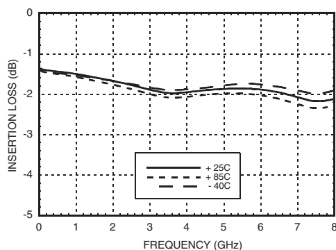
Insertion Loss
