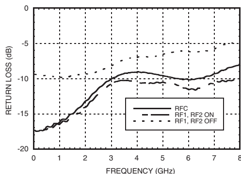
Return Loss
