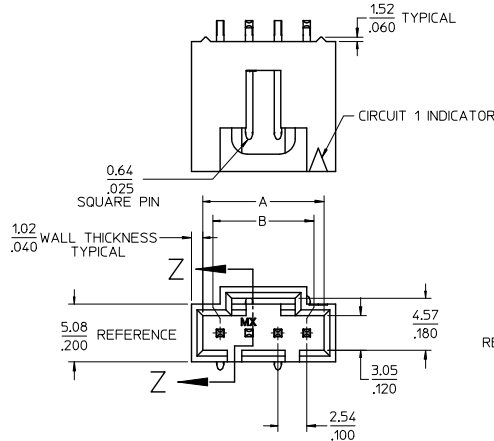
4 CIRCUIT SHOWN
