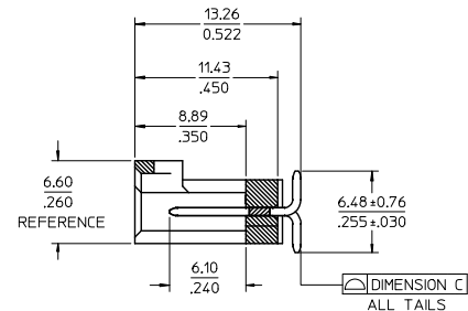
SECTION Z-Z
