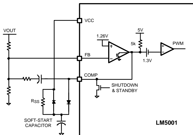
Figure 17. Soft-Start
