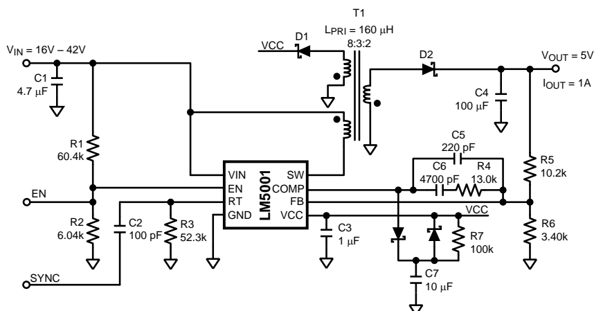
Figure 18. Non-Isolated Flyback
