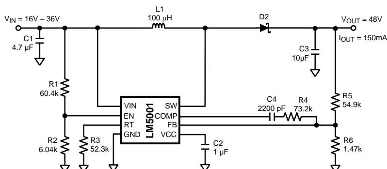
Figure 20. Boost
