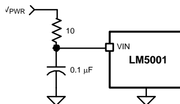
Figure 14. Input Transient Protection
