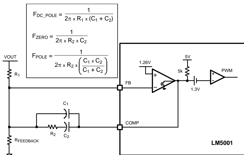
Figure 13. Type II Compensator
