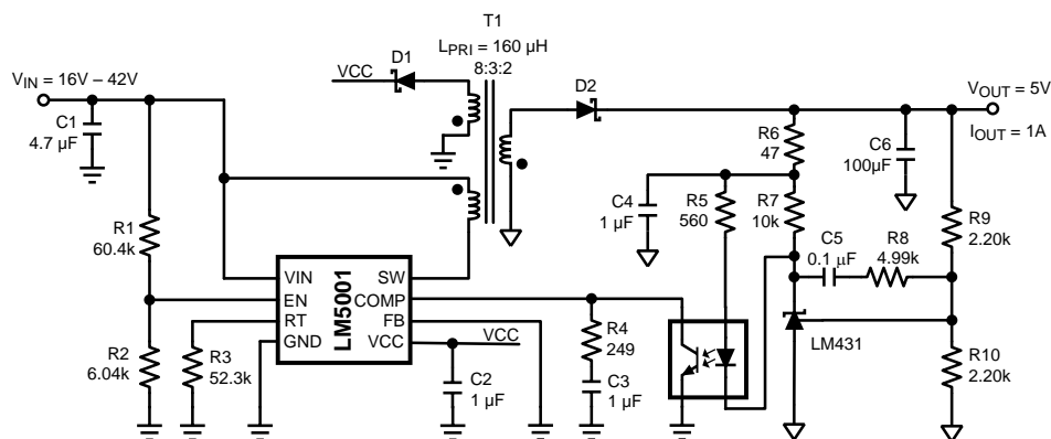
Figure 19. Isolated Flyback
