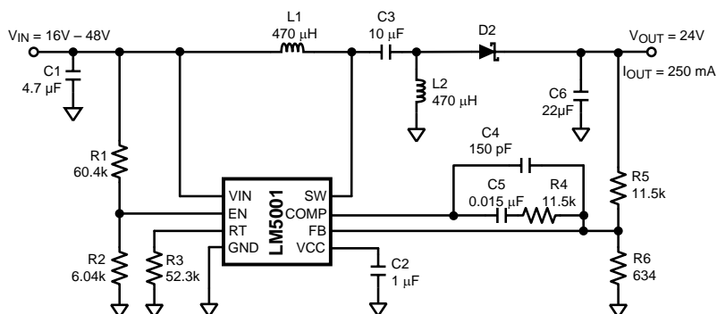
Figure 21. 24-V SEPIC
