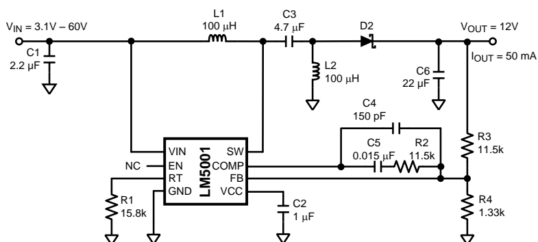
Figure 22. 12-V SEPIC
