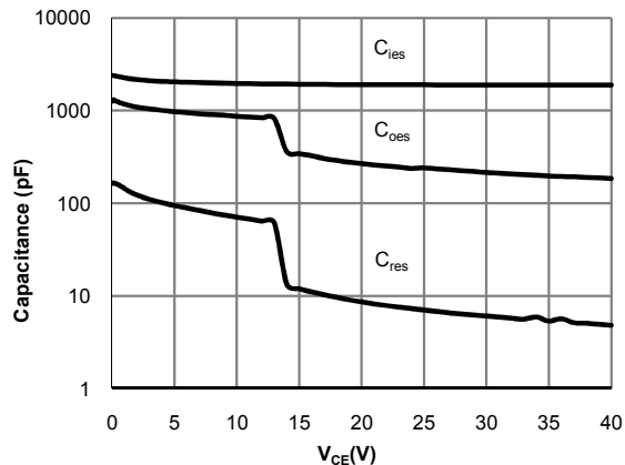
Fig 8: Capacitance Characteristic
