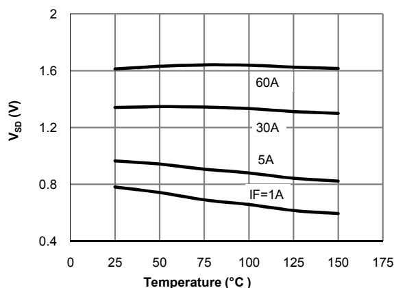
Fig 21: Diode Forward voltage vs. Junction Temperature
