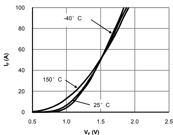
Fig 4: Diode Characteristic
