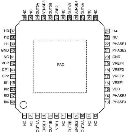
Package JP, 48-Pin LQFP Pin-out
