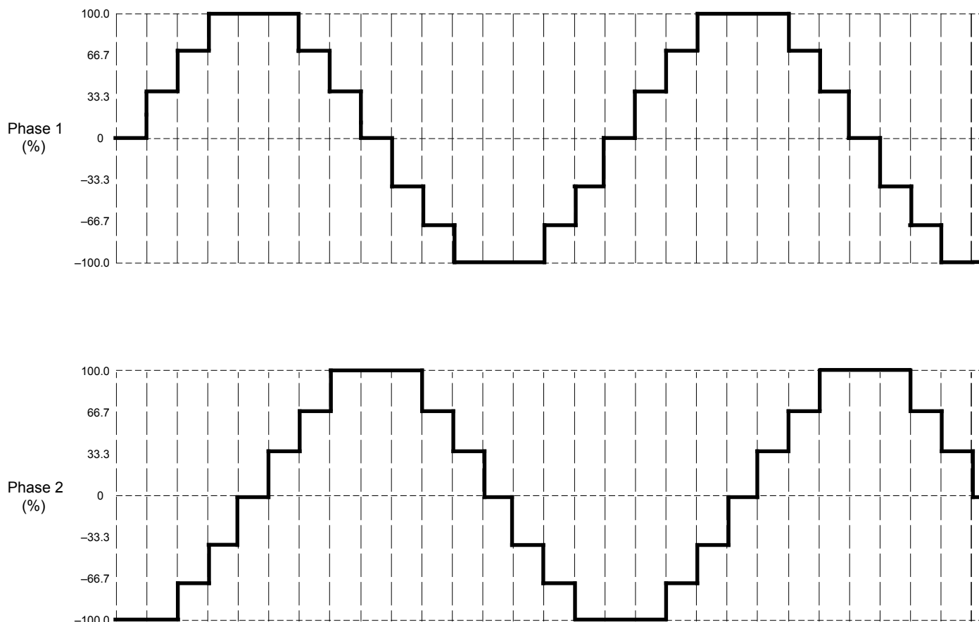
Figure 4: Step Sequence for Quarter-Step Increments
