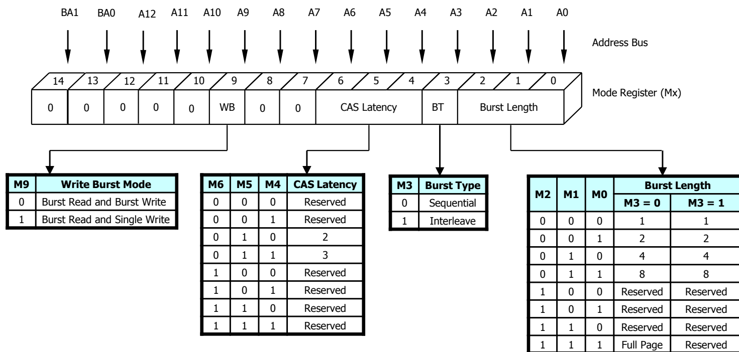
Figure4: Mode Register Definition
