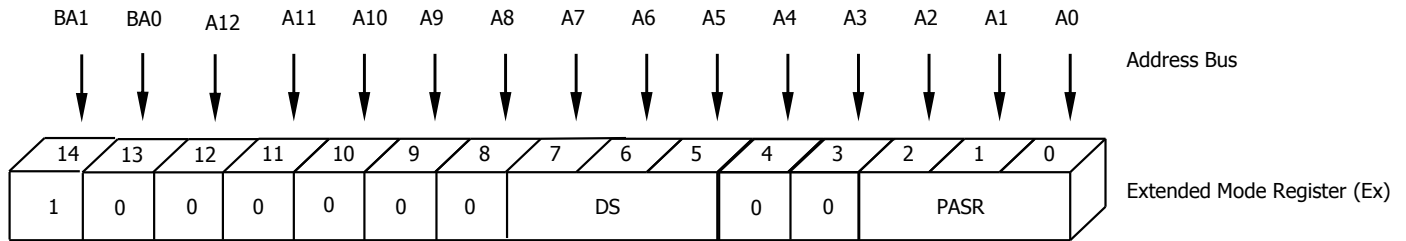
Figure5: Extended Mode Register
