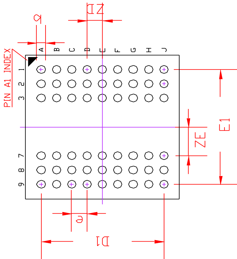
BOTTOM VIEW
