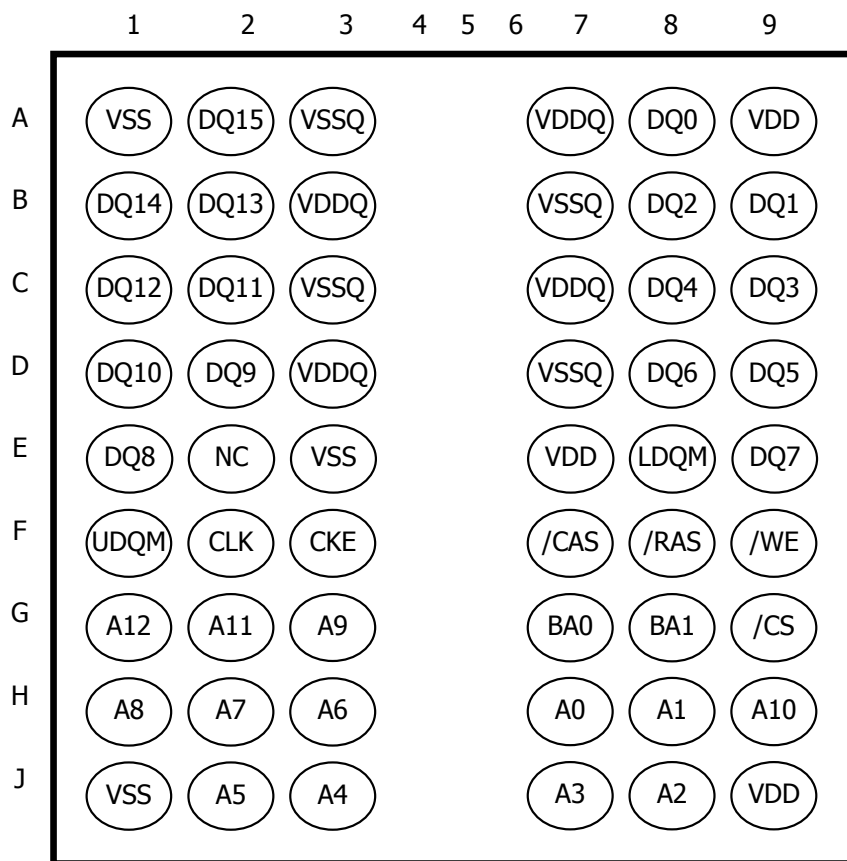
Figure1: 54Ball FBGA Ball Assignment
