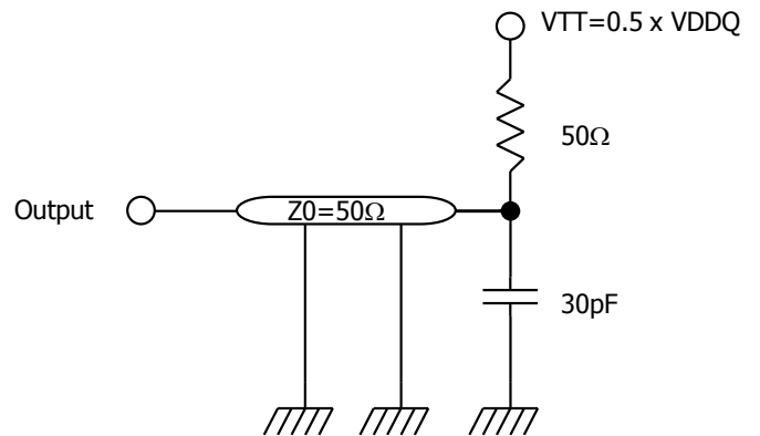
AC Output Load Circuit
