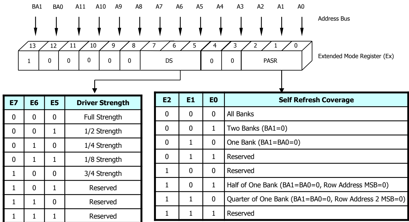
Figure5: Extended Mode Register
