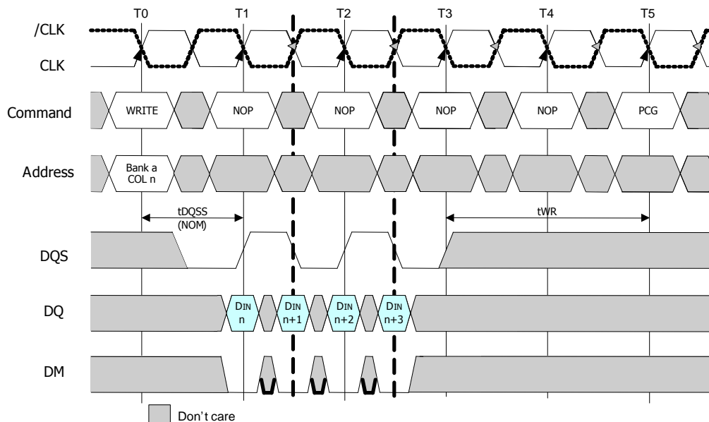
Figure29 : Write to Precharge (Uninterrupting)
