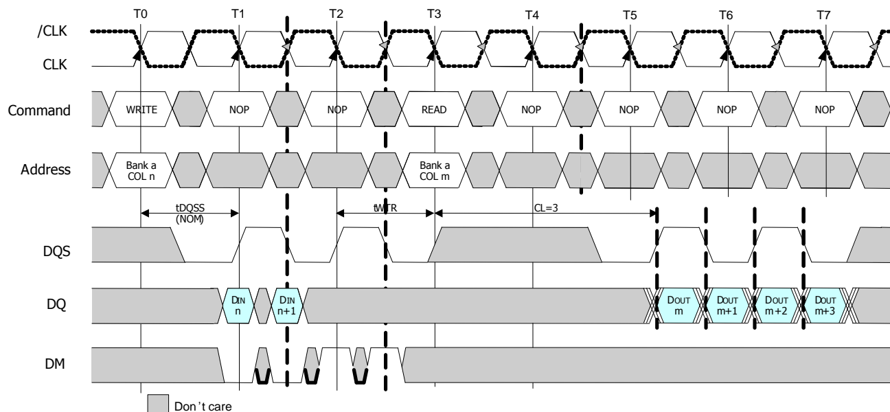
Figure27 : Write to Read (Interrupting)
