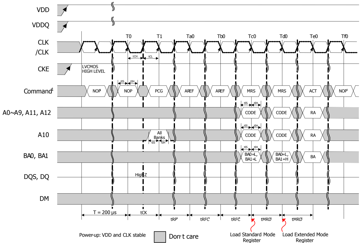
Figure6 : Power up sequence
