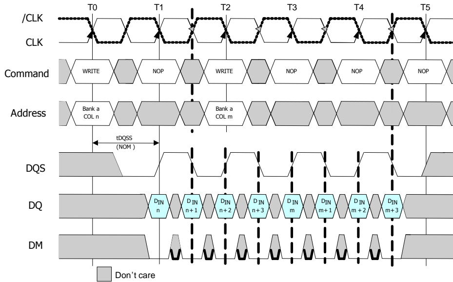
Figure23 : Consecutive Write to write (BL=4)
