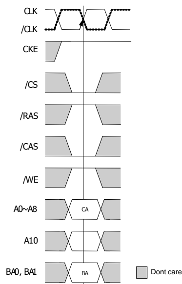
Figure14 : Read Data out timing (BL=4)
