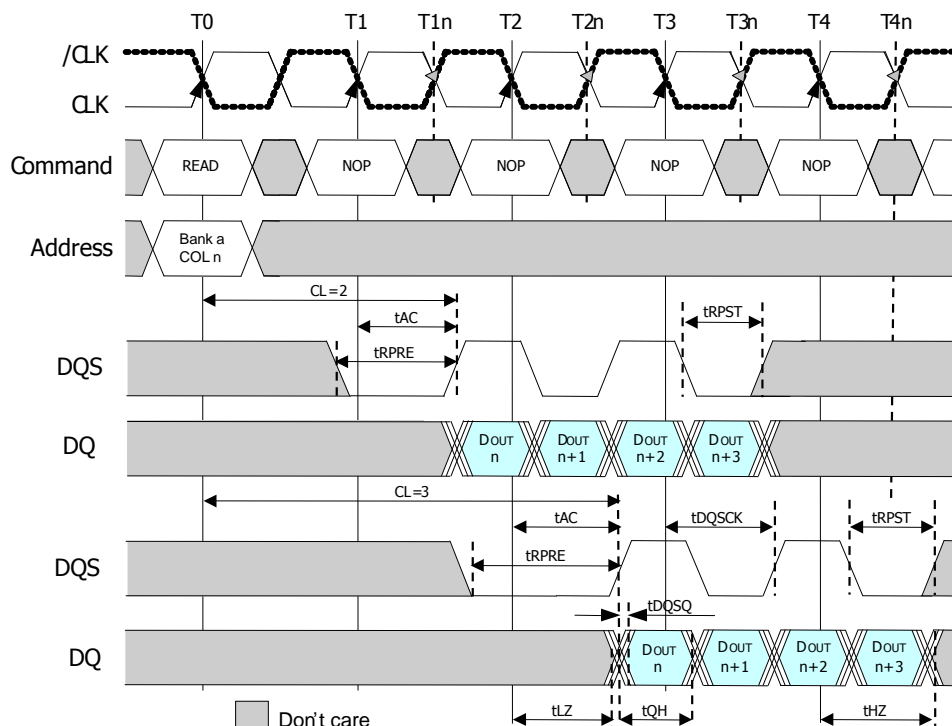
Figure14 : Read Data out timing (BL=4)
