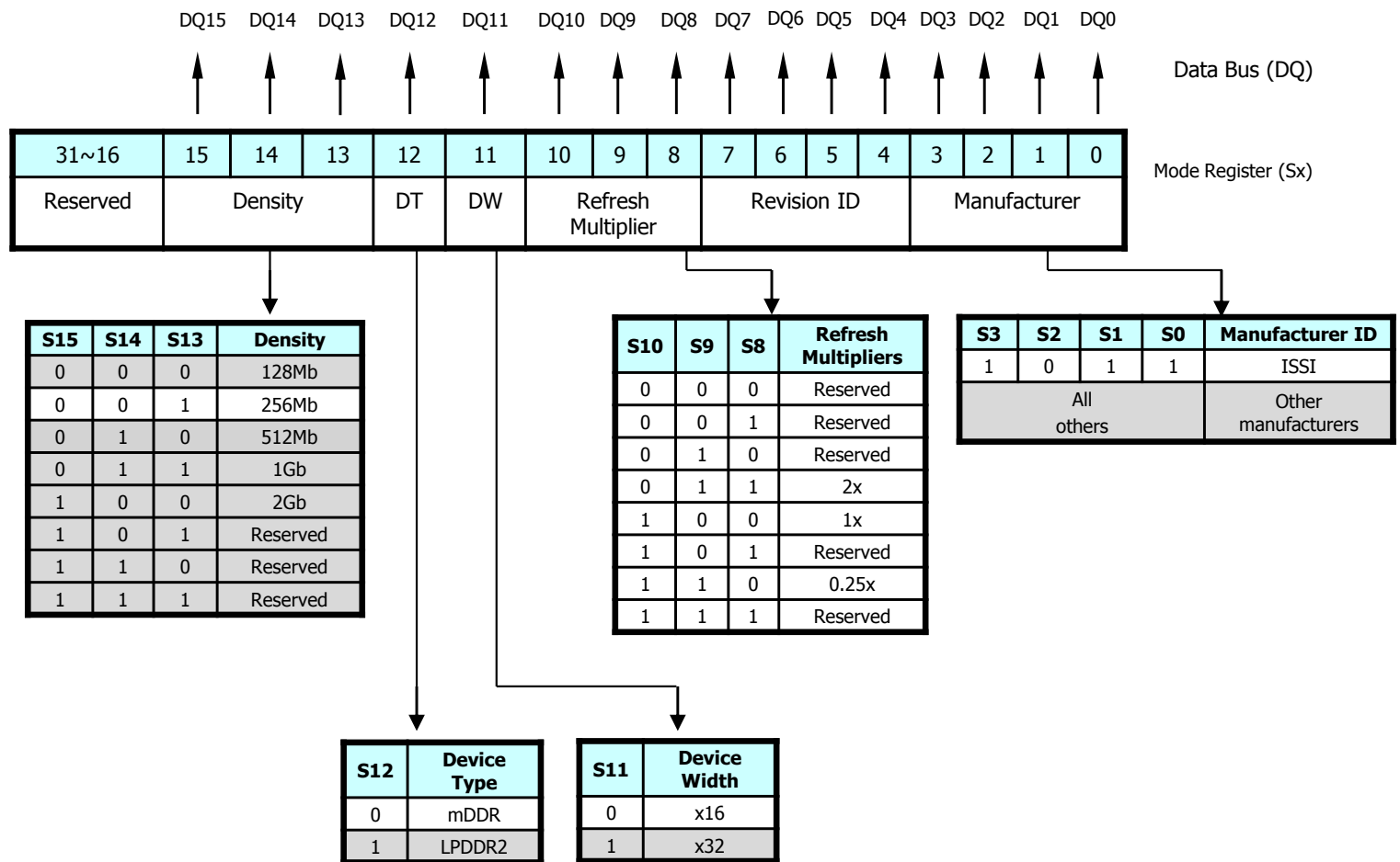
Figure8 : Status Register Read (SRR)
