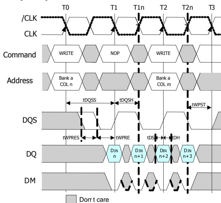
Figure22 : Write Burst (BL=4)
