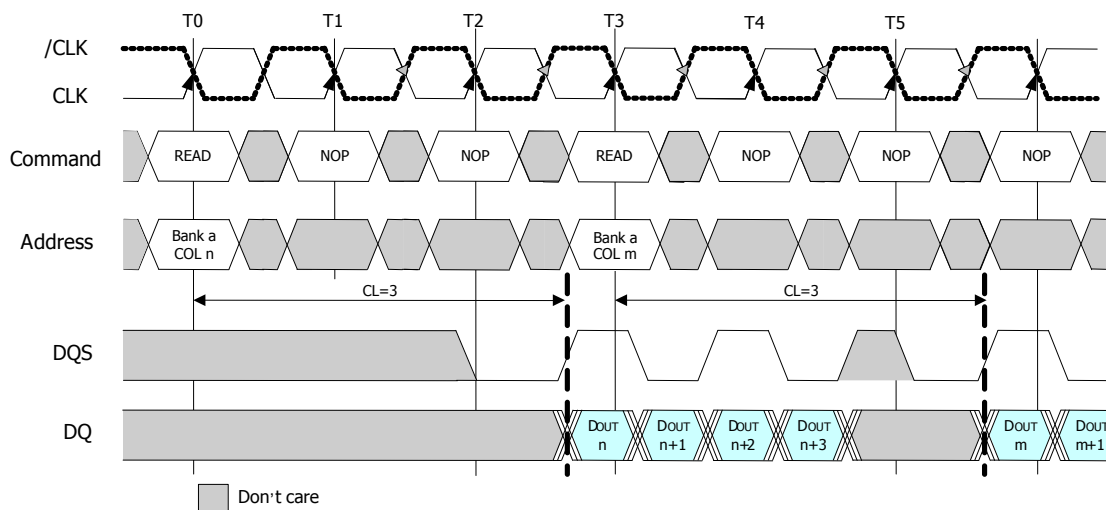
Figure16 : Non-Consecutive Read bursts (BL=4)
