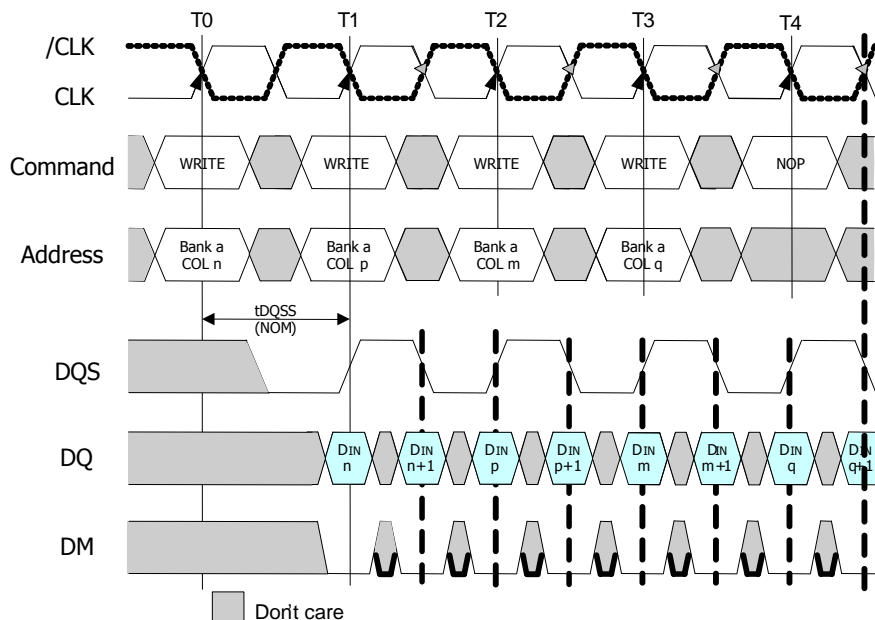
Figure25 : Random Write to write
