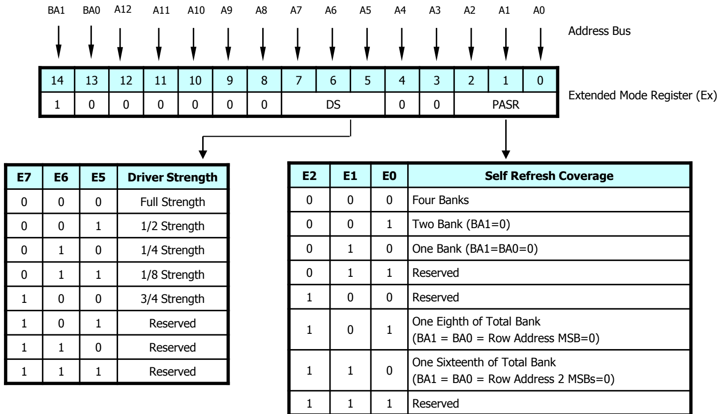
Figure5 : Extended Mode Set (EMRS) Register
