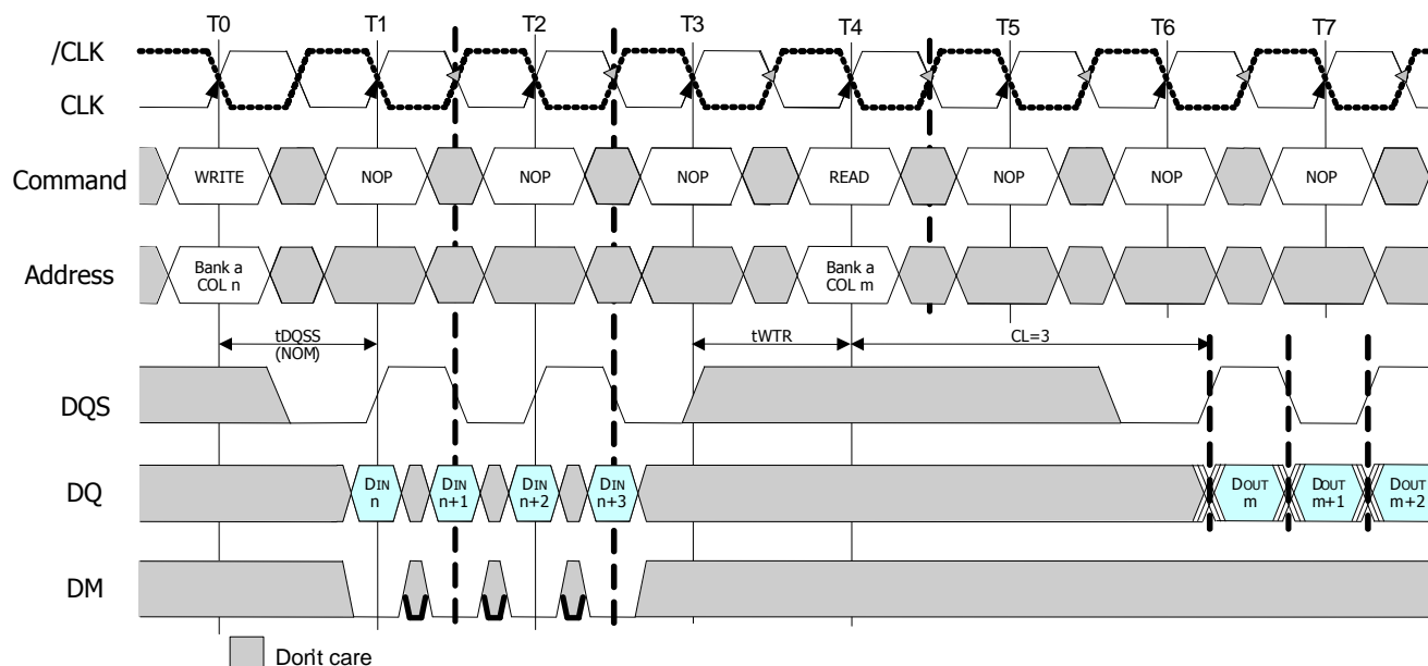
Figure26 : Write to Read (Uninterrupting)
