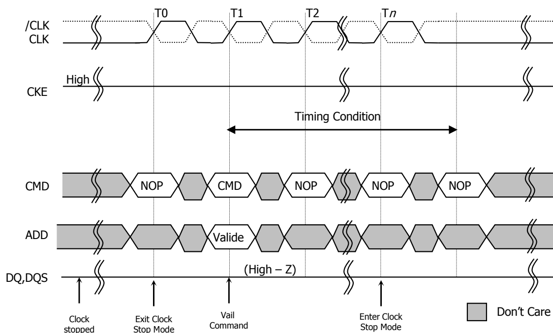
Figure 38 : Clock Stop Mode
