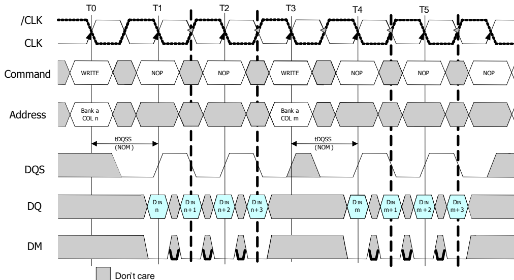
Figure24 : Non-Consecutive Write to write (BL=4)
