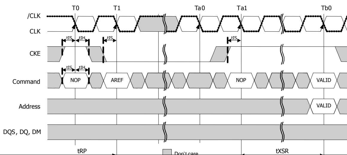
Figure35 : Self refresh
