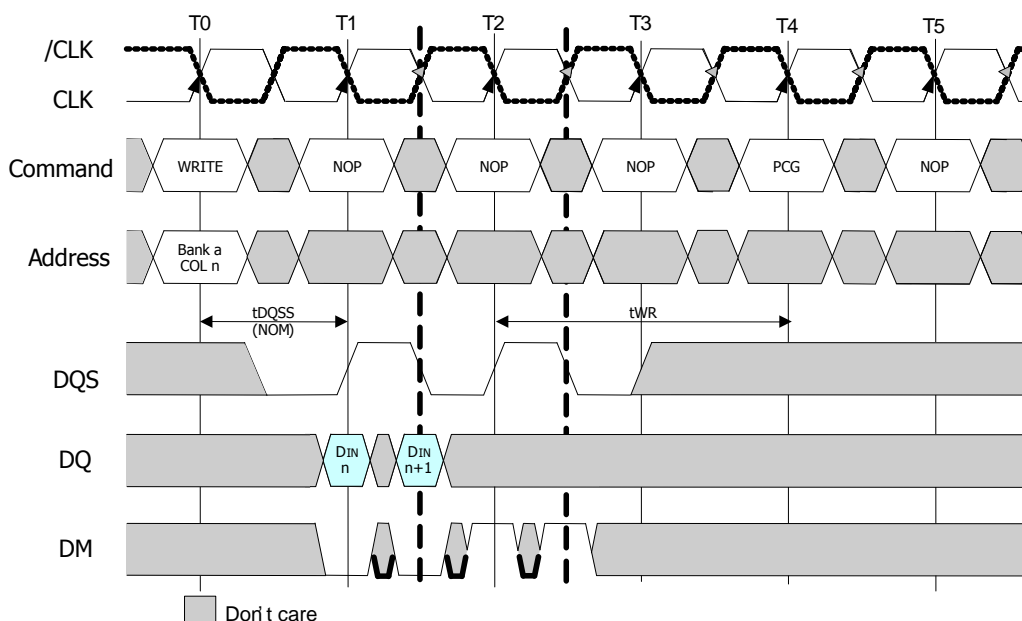
Figure30 : Write to Precharge (Interrupting)
