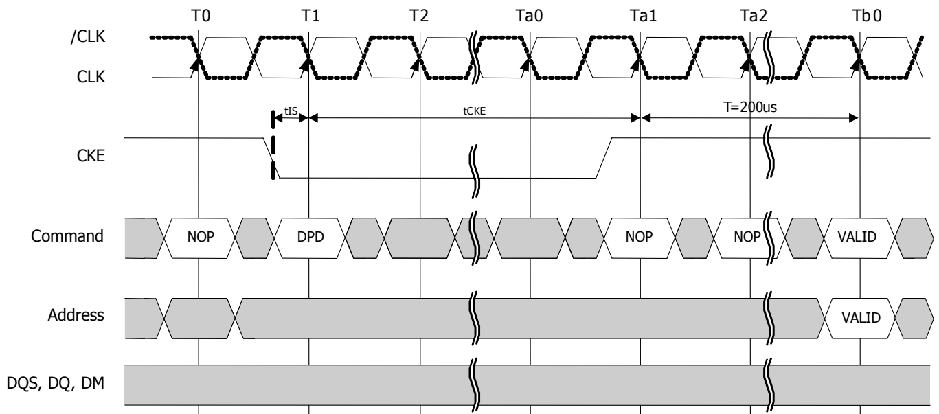
Figure37 : Deep Power down
