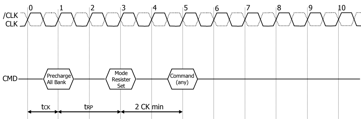
Figure33 : Mode Resister Set
