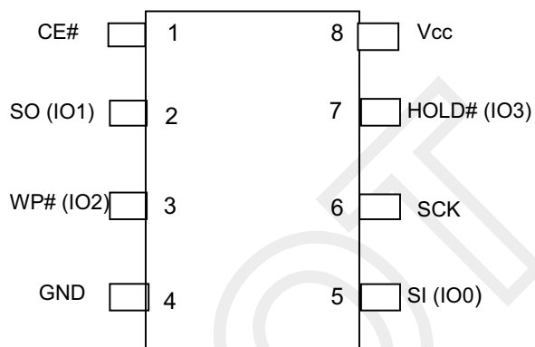
8-Pin SOIC/VVSOP
