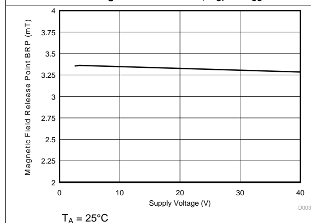
Figure 5. DRV5033AJ, B_{RP} vs V_{CC}
