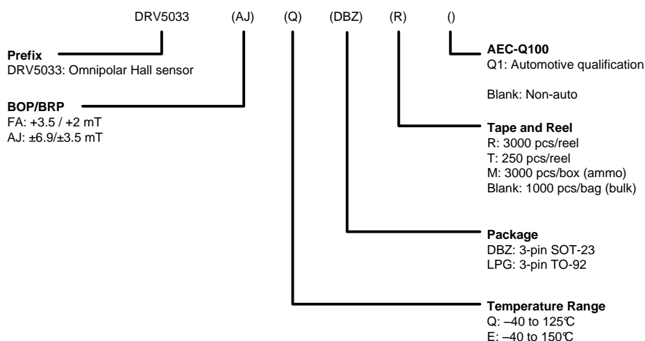
Figure 23. Device Nomenclature
