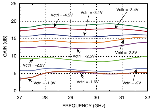
Gain vs. Control Voltage Range
