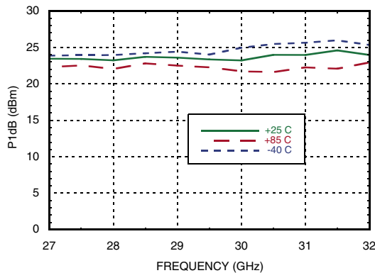
P1dB vs. Temperature, Vctrl= -4.5V
