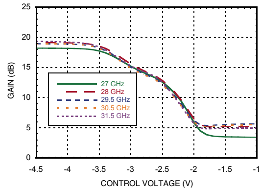
Gain vs. Control Voltage
