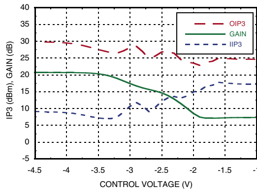
IP3 and Gain @ 31.5 GHz Pin = -7 dBm
