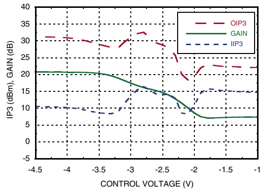
IP3 and Gain @ 29.5 GHz Pin = -7 dBm
