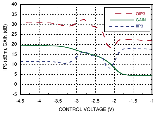
IP3 and Gain @ 27 GHz Pin = -7 dBm
