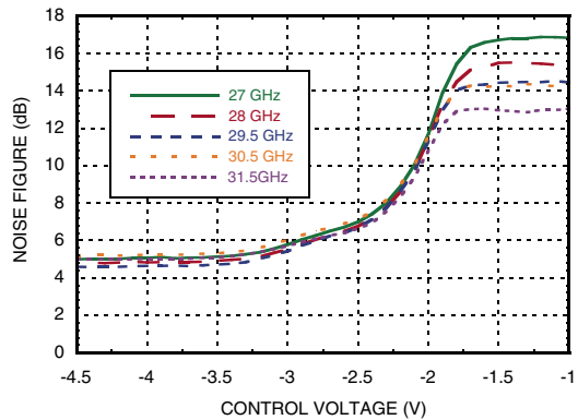
Noise Figure vs. Control Voltage
