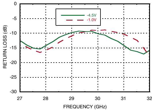
Input Return Loss @ Control Voltage Extreme
