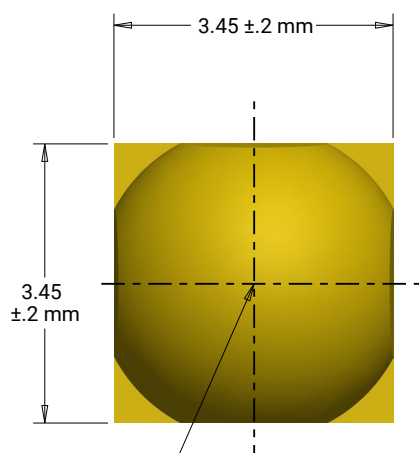
OPTICAL REFERENCE Top View
