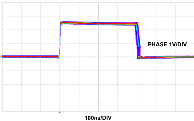
FIGURE 35. JITTER AT NO LOAD, PWM
