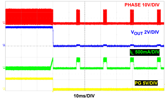
FIGURE 44. OVERCURRENT PROTECTION
