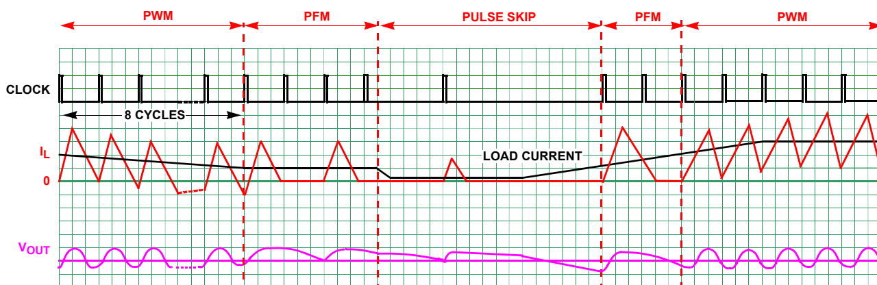
FIGURE 50. PFM MODE OPERATION WAVEFORMS
