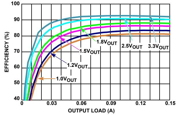
FIGURE 4. EFFICIENCY vs LOAD, PWM, V_{IN} = 5\text{V}
