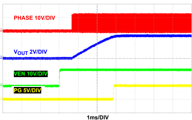
FIGURE 23. START-UP AT 150mA, PWM
