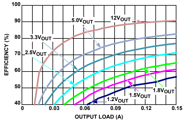
FIGURE 10. EFFICIENCY vs LOAD, PWM, V_{IN} = 36V
