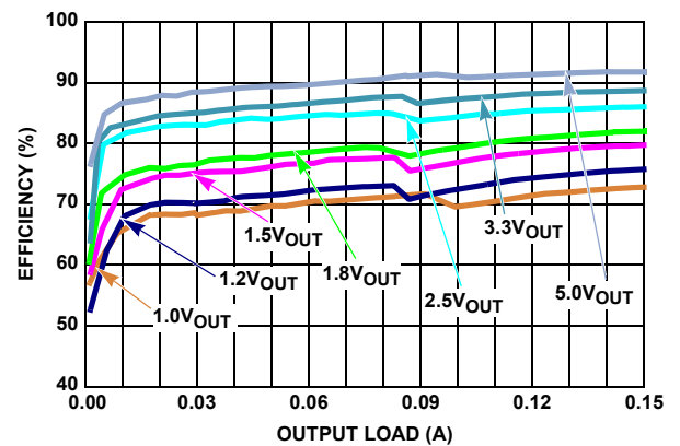
FIGURE 2. EFFICIENCY vs LOAD, PFM, V_{IN} = 12\text{V}
