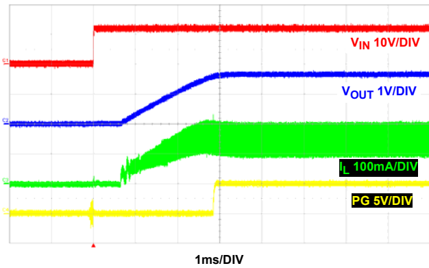
FIGURE 27. START-UP V_{IN} AT 150mA LOAD, PFM
