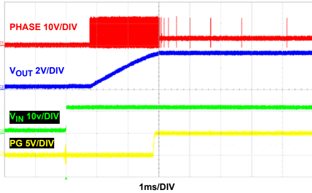
FIGURE 31. START-UP V_{IN} AT NO LOAD, PFM
