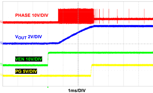
FIGURE 19. START-UP AT NO LOAD, PFM
