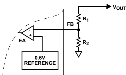
FIGURE 51. EXTERNAL RESISTOR DIVIDER
