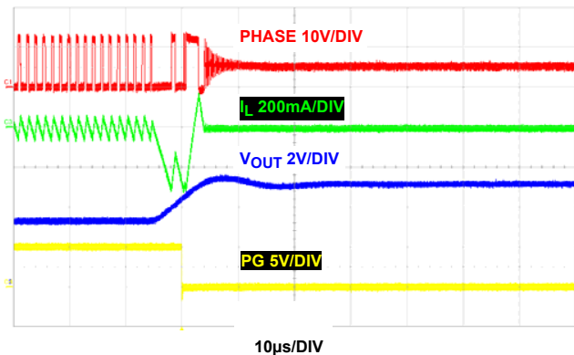
FIGURE 47. OVERVOLTAGE PROTECTION
