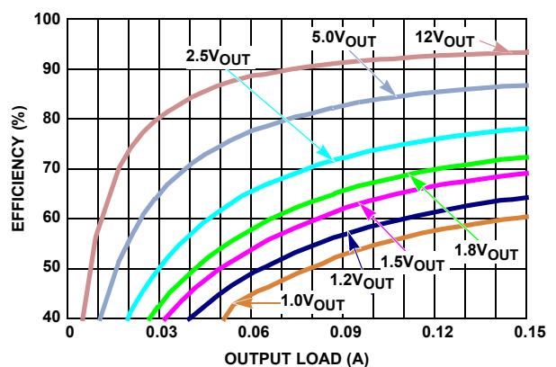
FIGURE 8. EFFICIENCY vs LOAD, PWM, V_{IN} = 24\text{V}
