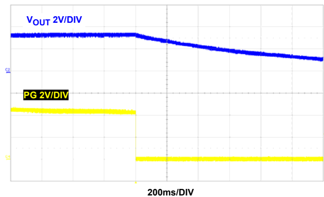
FIGURE 48. OVERTEMPERATURE PROTECTION
