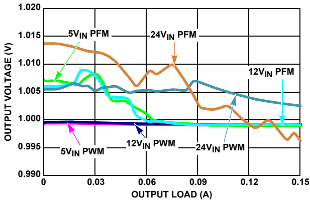
FIGURE 11. V_{OUT} REGULATION vs LOAD, V_{OUT} = 1V
