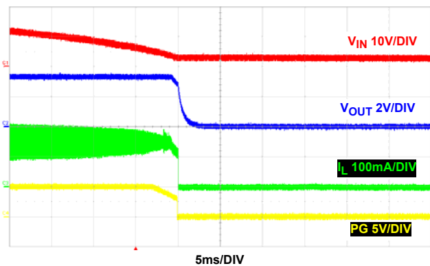
FIGURE 29. SHUTDOWN V_{IN} AT 150mA LOAD, PFM
