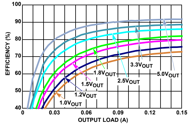
FIGURE 6. EFFICIENCY vs LOAD, PWM, V_{IN} = 12\text{V}
