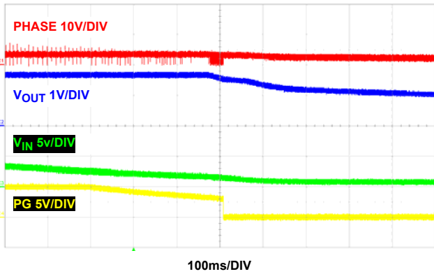
FIGURE 33. SHUTDOWN V_{IN} AT NO LOAD, PFM
