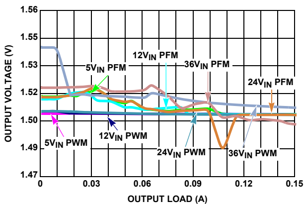
FIGURE 13. V_{OUT} REGULATION vs LOAD, PWM, V_{OUT} = 1.5V
