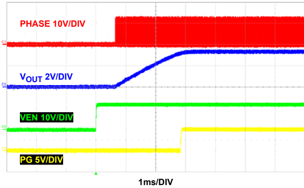
FIGURE 25. START-UP AT 150mA, PFM
