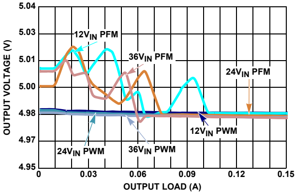
FIGURE 17. V_{OUT} REGULATION vs LOAD, V_{OUT} = 5V
