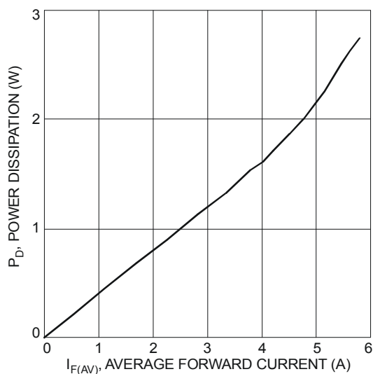
Figure 1 Forward Power Dissipation
