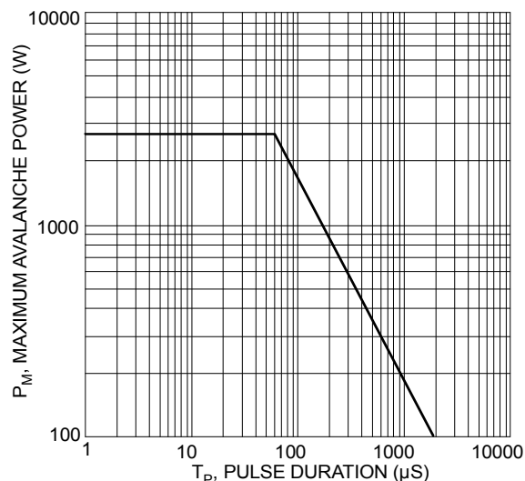
Figure 8 Maximum Avalanche Power
