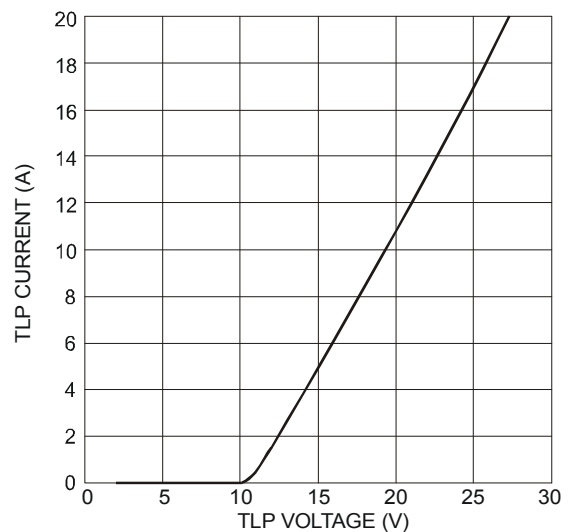
Figure 8 Transmission Line Pulsing (TLP) Current vs. Voltage
