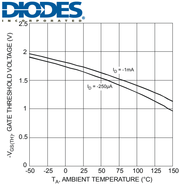
Figure 7 Gate Threshold Variation vs. Ambient Temperature
