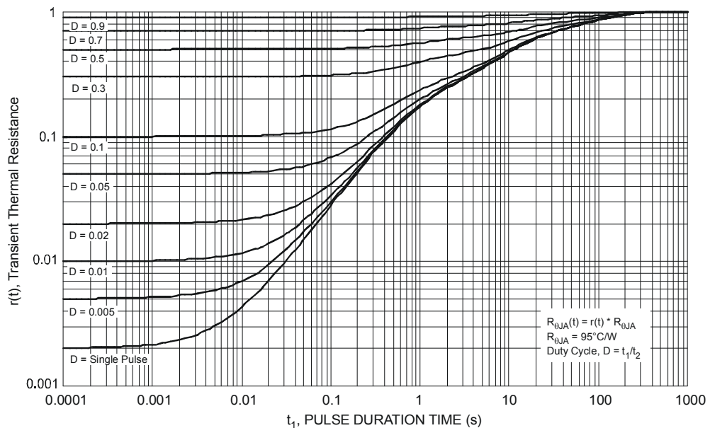
Figure 11 Transient Thermal Response
