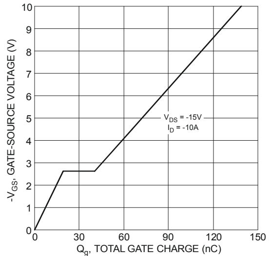
Figure 10 Gate-Source Voltage vs. Total Gate Charge
