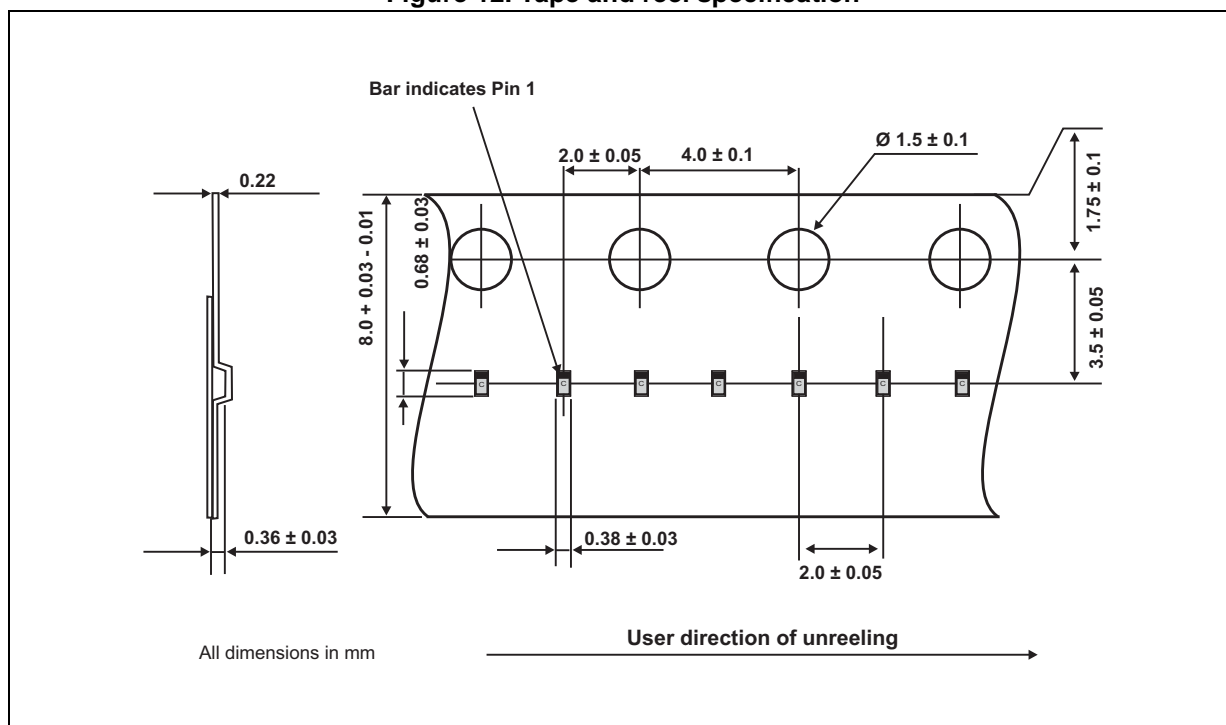
Figure 12. Tape and reel specification
