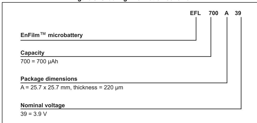
Figure 8. Ordering information scheme
