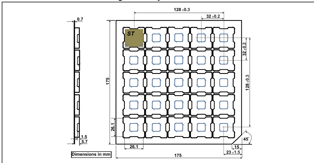
Figure 6. Tray dimensions
