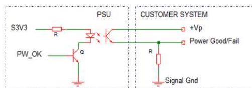
Figure 6: Isolated Signal Output connections
