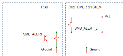
Figure 6: Isolated Signal Output connections
