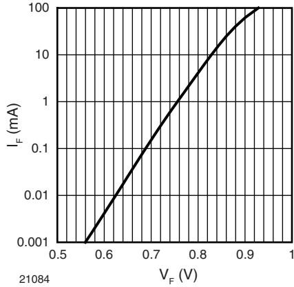
Fig. 3 - Typical Forward Current I_F vs. Forward Voltage V_F
