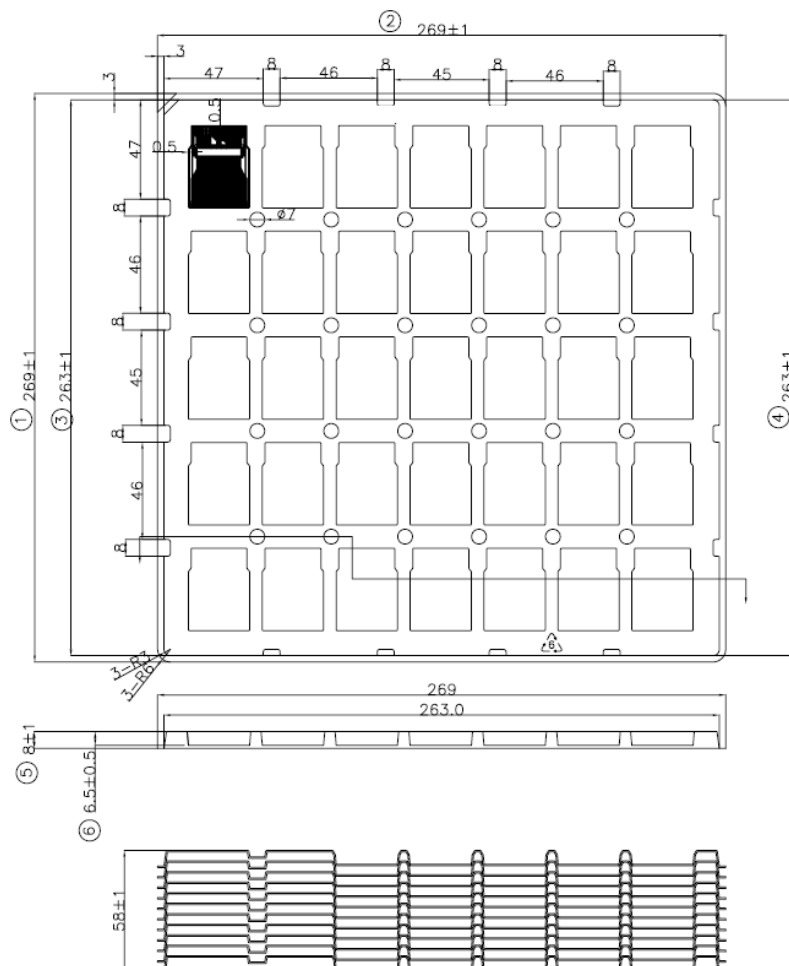
Figure 1. TDS Tray Dimensions
