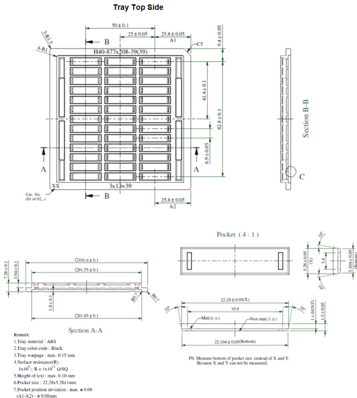
Figure 3. GBTD Die Tray Dimension Details
