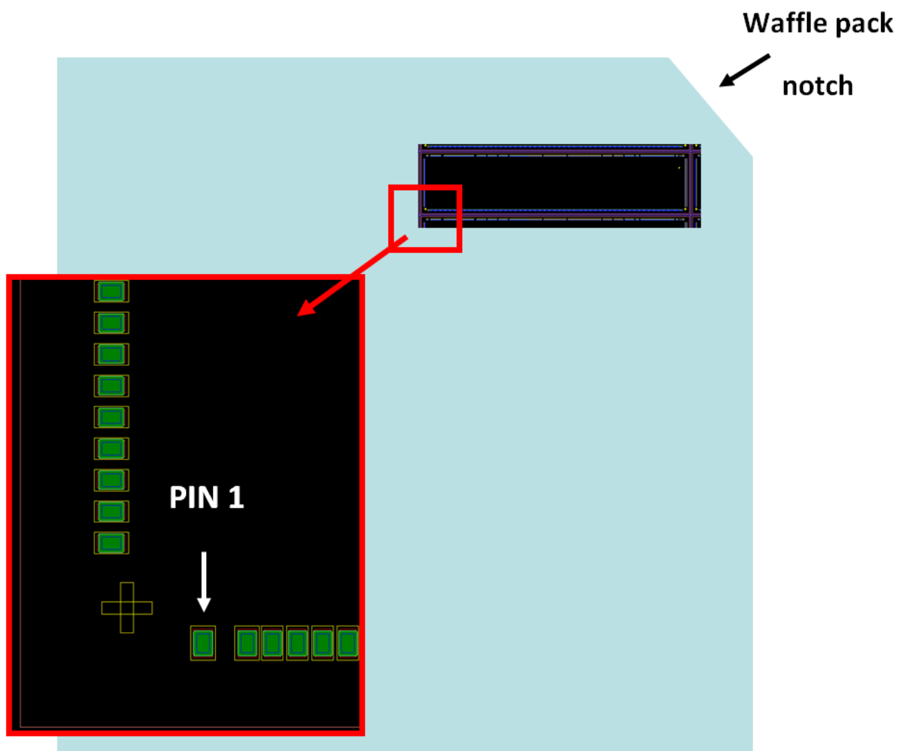
Figure 4. GBTD Die, Pin 1 Location
