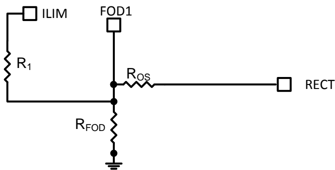
Figure 15. Current Limit Setting for bq5102x
