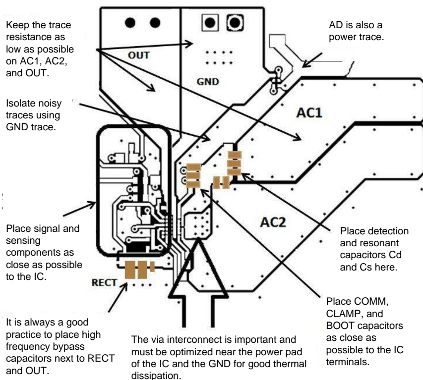
Figure 29. Layout Example for bq5102x
