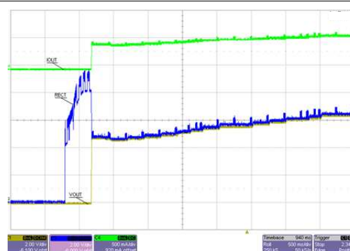
Figure 25. Output Regulation on a WPC TX
