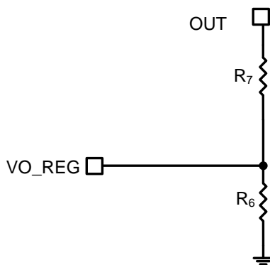
Figure 8. VO_REG Network
