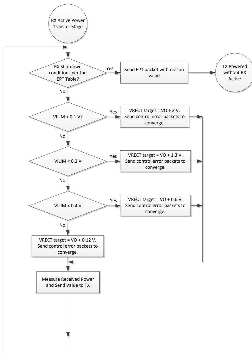
Figure 12. Active Power Transfer Flow Diagram on WPC
