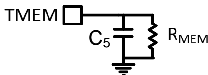
Figure 9. TMEM Configuration
