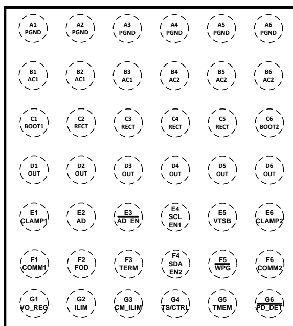
Pin Functions
