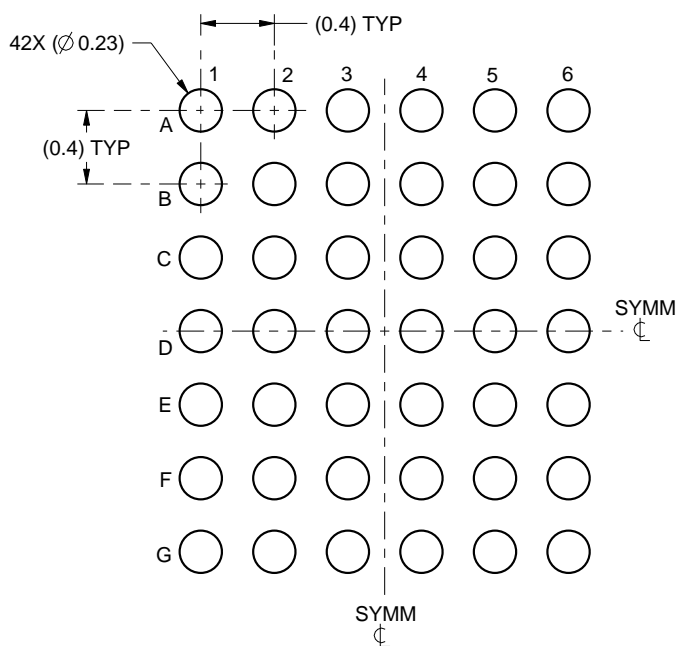
LAND PATTERN EXAMPLE SCALE:25X
