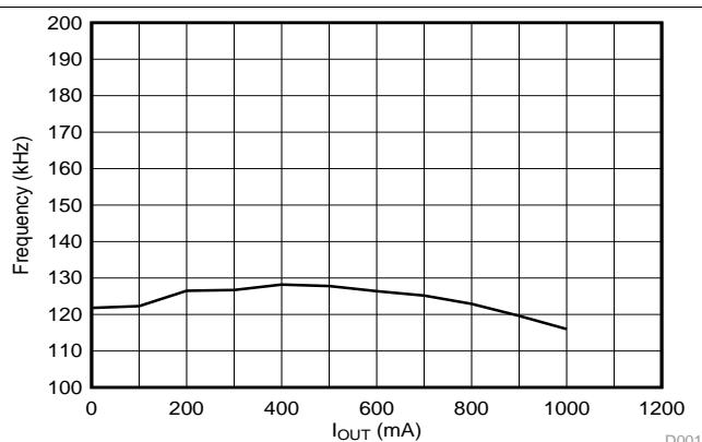
Figure 23. Frequency Range of 5-V, 1-A RX on a WPC TX
