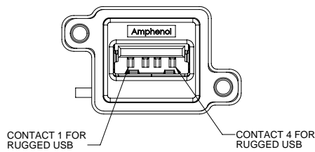
MUSB CONTACT ASSIGNMENT
