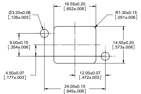
RECOMMENDED PANEL CUTOUT (OUTSIDE VIEW OF PANEL)
