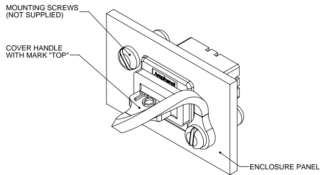
DUST COVER APPLICATION
