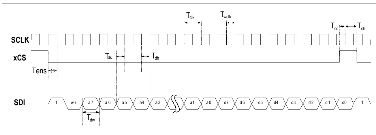
Figure 1-3. Serial WRITE Mode
