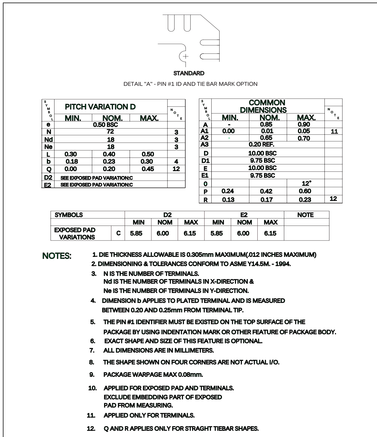
Figure 2-10. 72-Pin Package Dimensions
