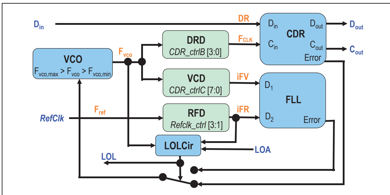
Figure 1-8. Block Diagram of Frequency Acquisition Circuits
