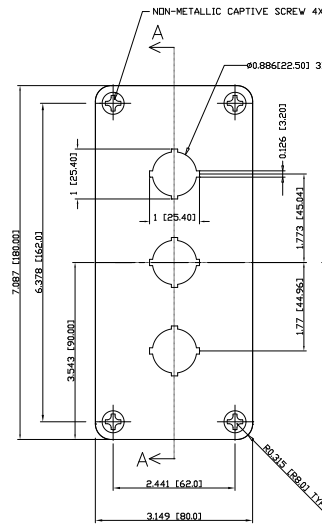
TOP VIEW WITH COVER
