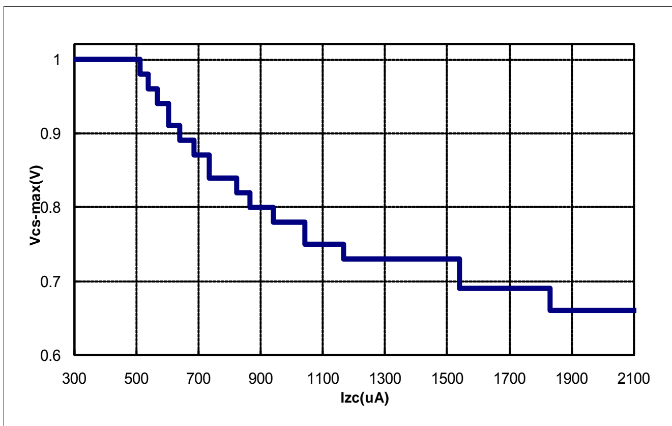
Figure 7 VCS-max versus IZC
