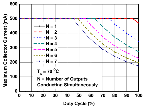
Figure 14 Maximum Collector Current vs. Duty Cycle
