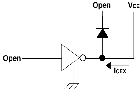
Fig.1 ICEX Test Circuit
