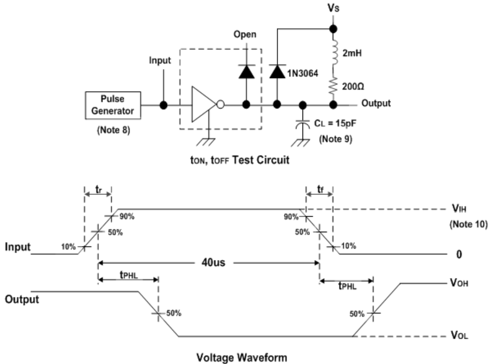
Fig. 10 Latch-Up Test Circuit and Voltage Waveform
