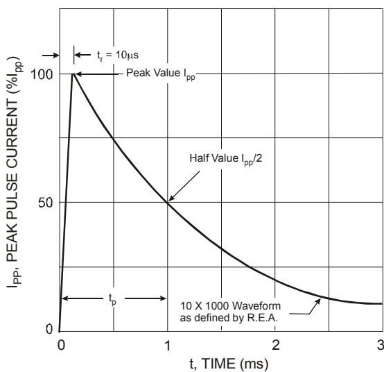
Figure 1 Pulse Waveform
