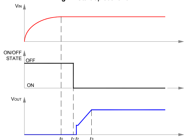
Fig. 8: Start-up scenario #2.
