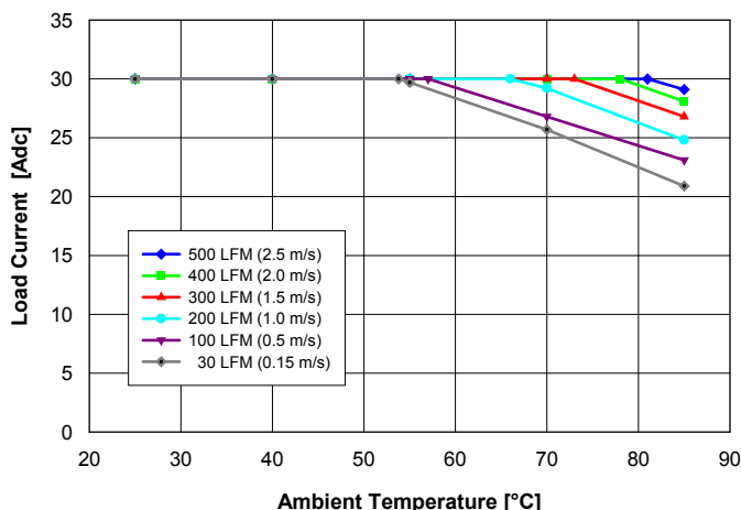
Fig. 1: Available load current vs. ambient air temperature and air-flow rates for Q48S30015 converter mounted vertically with air flowing from pin 3 to pin 1, MOSFET temperature \leq 120^{\circ}\text{C} , V_{in} = 54\text{ V} .
