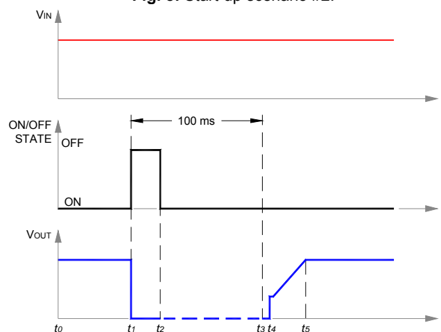
Fig. 9: Start-up scenario #3.
