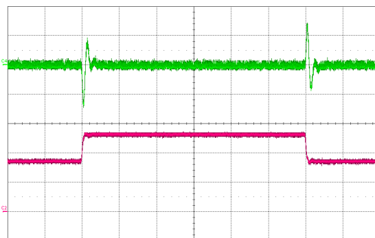
Fig. 30: Output voltage response to load current step-change (17.5 A – 26.25 A – 17.5 A) at V_{in} = 48\text{ V} . Top trace: output voltage (200 mV/div.). Bottom trace: load current (10 A/div.). Current slew rate: 1 A/ \mu\text{s} . C_o = 1\text{ }\mu\text{F} ceramic + 10 \mu\text{F} tantalum. Time scale: 200 \mu\text{s} /div.
