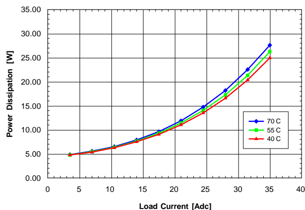
Fig. 26: Power dissipation vs. load current and ambient temperature for converter w/o baseplate mounted vertically with V_{in} = 48\text{ V} and air flowing from pin 3 to pin 1 at a rate of 200 LFM (1.0 m/s).
