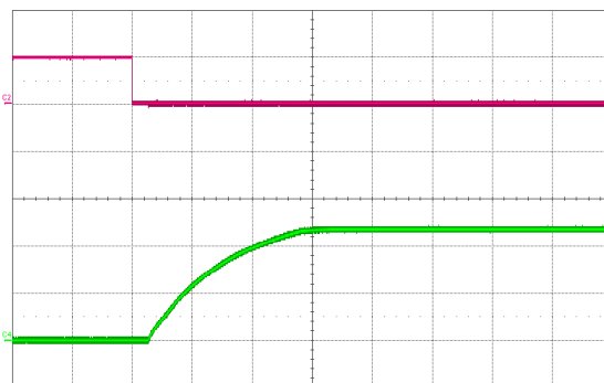
Fig. 28: Turn-on transient at full rated load current (resistive) plus 20,000 \mu\text{F} at V_{in} = 48\text{ V} , triggered via ON/OFF pin. Top trace: ON/OFF signal (5 V/div.). Bottom trace: output voltage (5 V/div.). Time scale: 5 ms/div.
