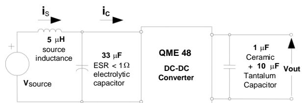
Fig. 32: Test setup for measuring input reflected ripple currents, i_c and i_s .
