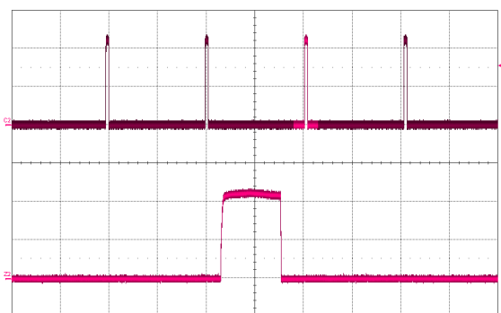
Fig. 35: Load current (top trace, 20 A/div., 100 ms/div.) into a 10 m \Omega short circuit during restart, at V_{in} = 48 \text{ V} . Bottom trace (20 A/div., 100 ms/div.) is an expansion of the on-time portion of the top trace.
